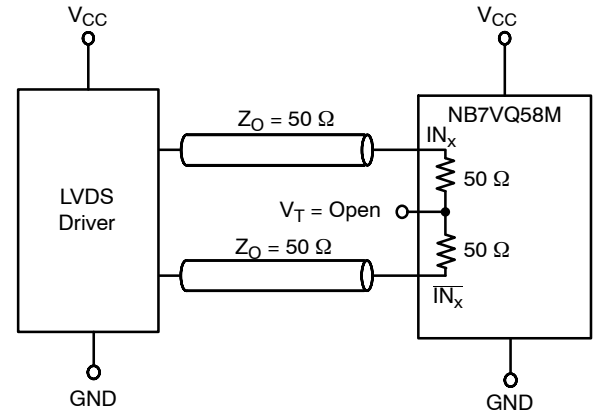
Figure 14. LVDS Interface
