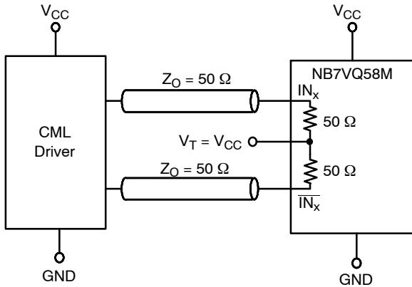
Figure 15. Standard 50 Ω Load CML Interface
