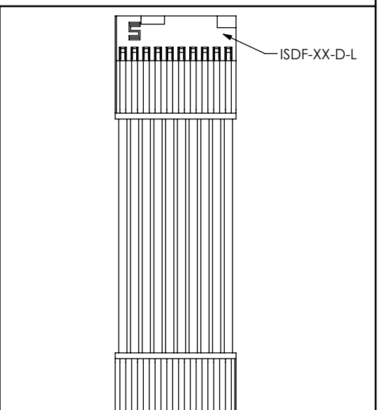
FIG 4 -DL: DOUBLE END FRICTION LOCK SFSDX-10-28-XX-XX.XX-DL-NUS SHOWN (SAME AS FIG 1, UNLESS OTHERWISE STATED)
