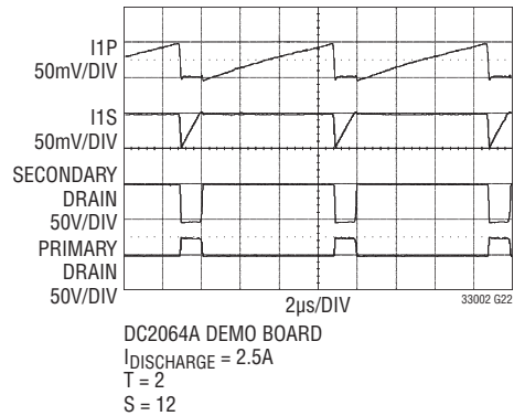
Typical Discharge Waveforms
