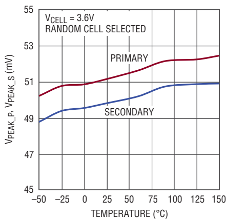
Peak Current Sense Threshold vs Temperature
