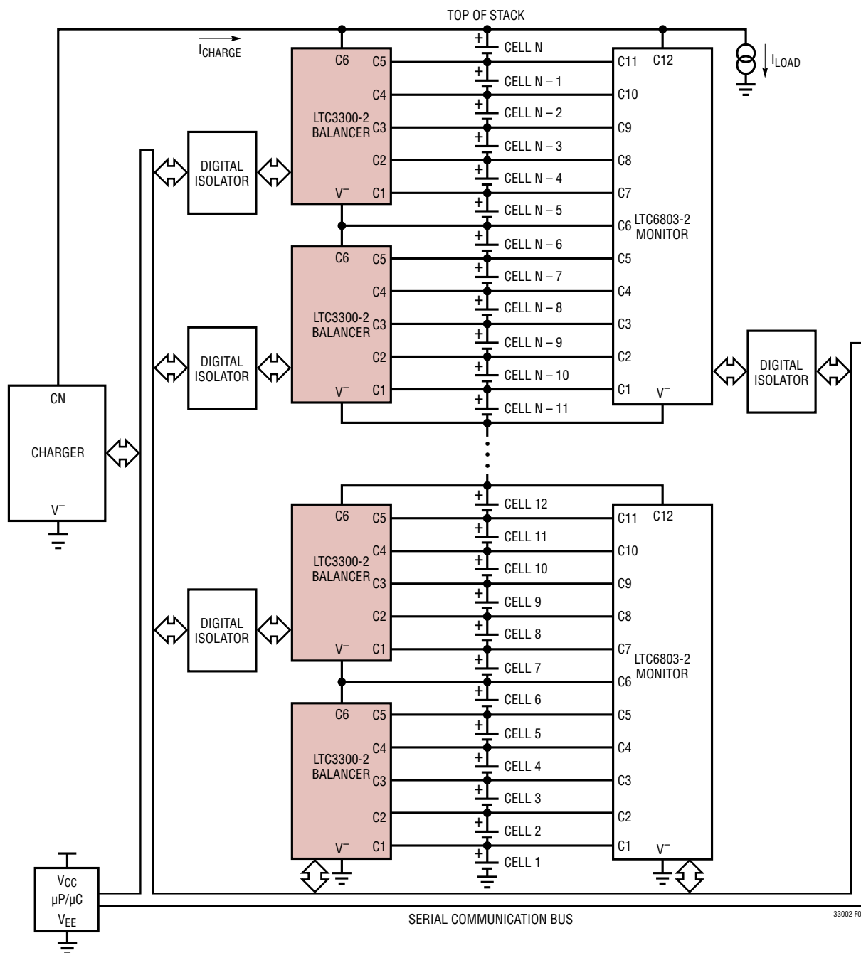
Figure 1. LTC3300-2/LTC6803-2 Typical Battery Management System (BMS)
