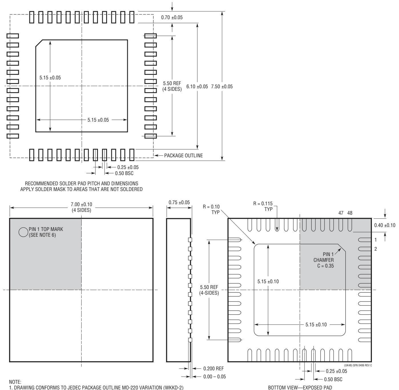
UK Package 48-Lead Plastic QFN (7mm × 7mm) (Reference LTC DWG # 05-08-1704 Rev C)
