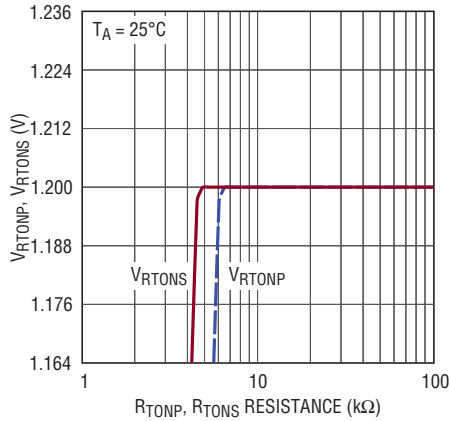
V_{RTONP} , V_{RTONS} vs External Resistance
