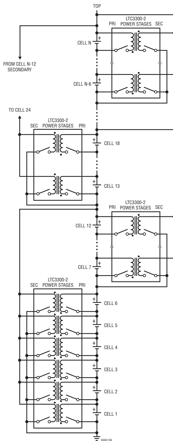
Figure 4. Diagram of Power Transfer Interleaving Through the Stack, Transformer Connections for High Voltage Stacks
