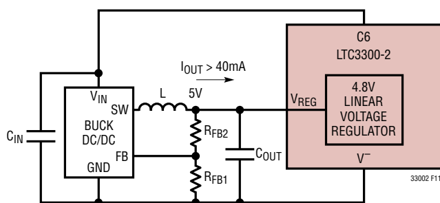
Figure 11. Adding External Buck DC/DC for >40mA V_{REG} Drive
