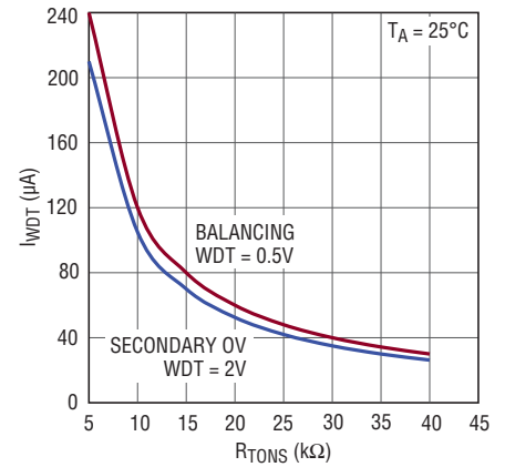
WDT Pin Current vs R_{TONS}
