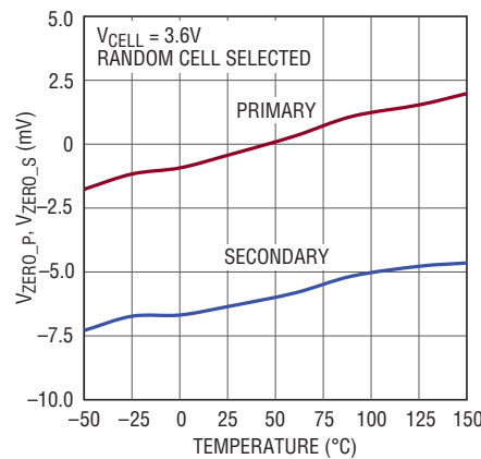
Zero Current Sense Threshold vs Temperature
