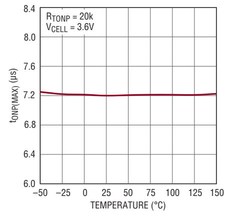
Primary Winding Switch Maximum On-Time vs Temperature
