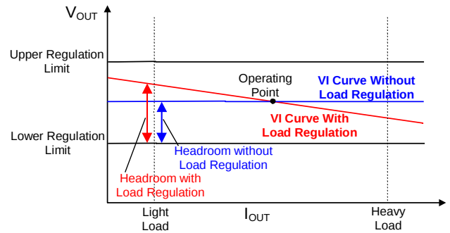
Figure 29. Concept of Optimal Voltage Positioning
