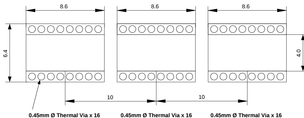
Figure 59. Recommended Pad Sizes
