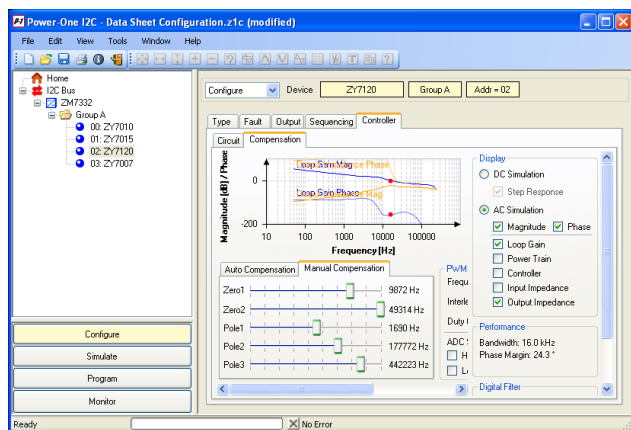
Figure 47. POL Configure Controller Compensation Window
