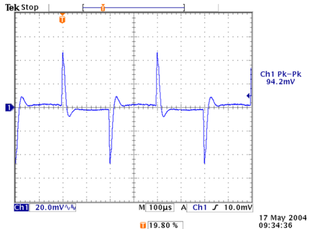
Figure 30. Transient Response without Optimal Voltage Positioning
