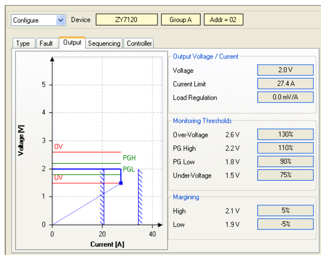
Figure 27. POL Configure Output Window
