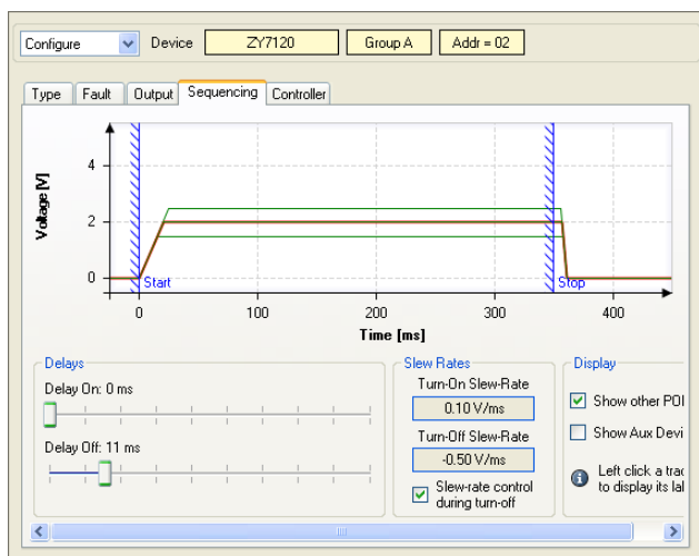
Figure 32. POL Configure Sequencing Window
