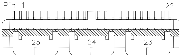
Figure 58. Pinout Diagram (Bottom View)
