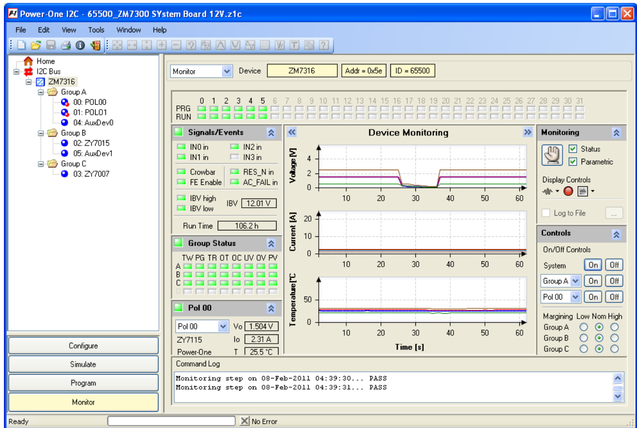
Figure 56. DPM Monitoring Window
