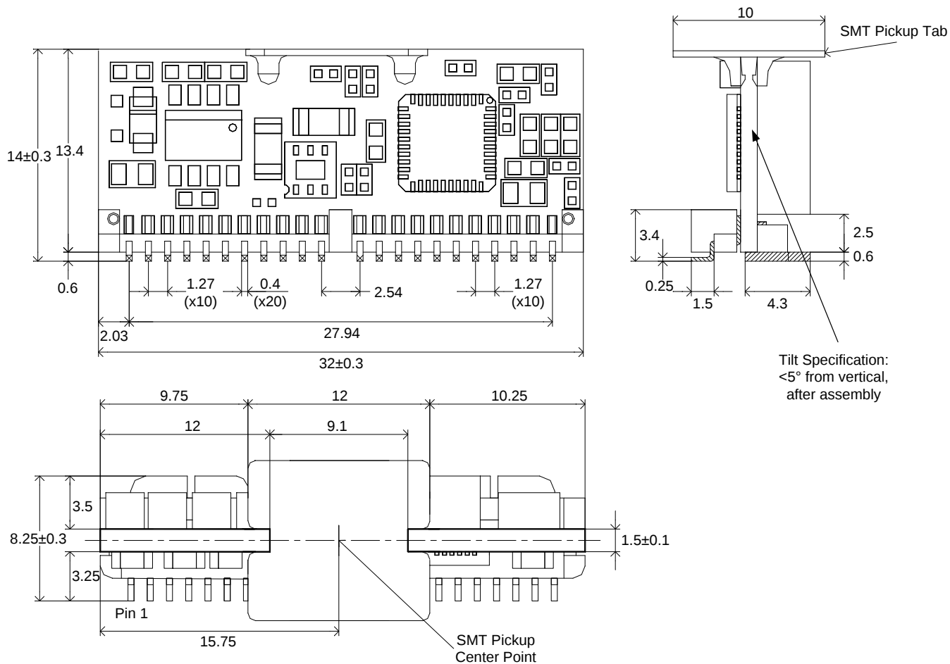
Figure 57. Mechanical Drawing
