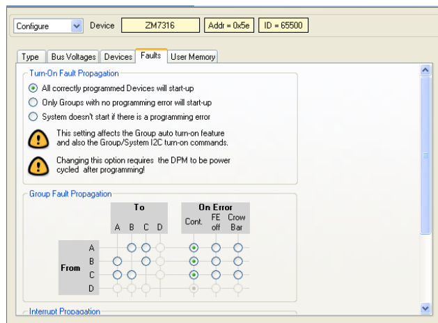
Figure 44. DPM Configure Faults Window
