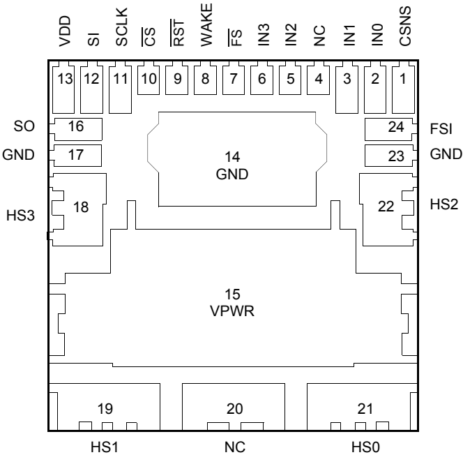
Figure 19. Pin Connections
