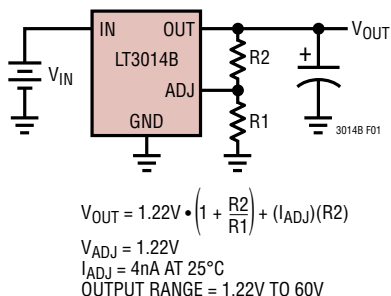
Figure 1. Adjustable Operation
