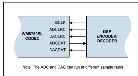
Figure 17 Slave Mode
