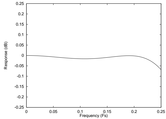
Figure 34 DAC Digital Filter Ripple – Type 3
