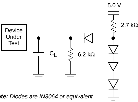
Figure 7. Test Setup
