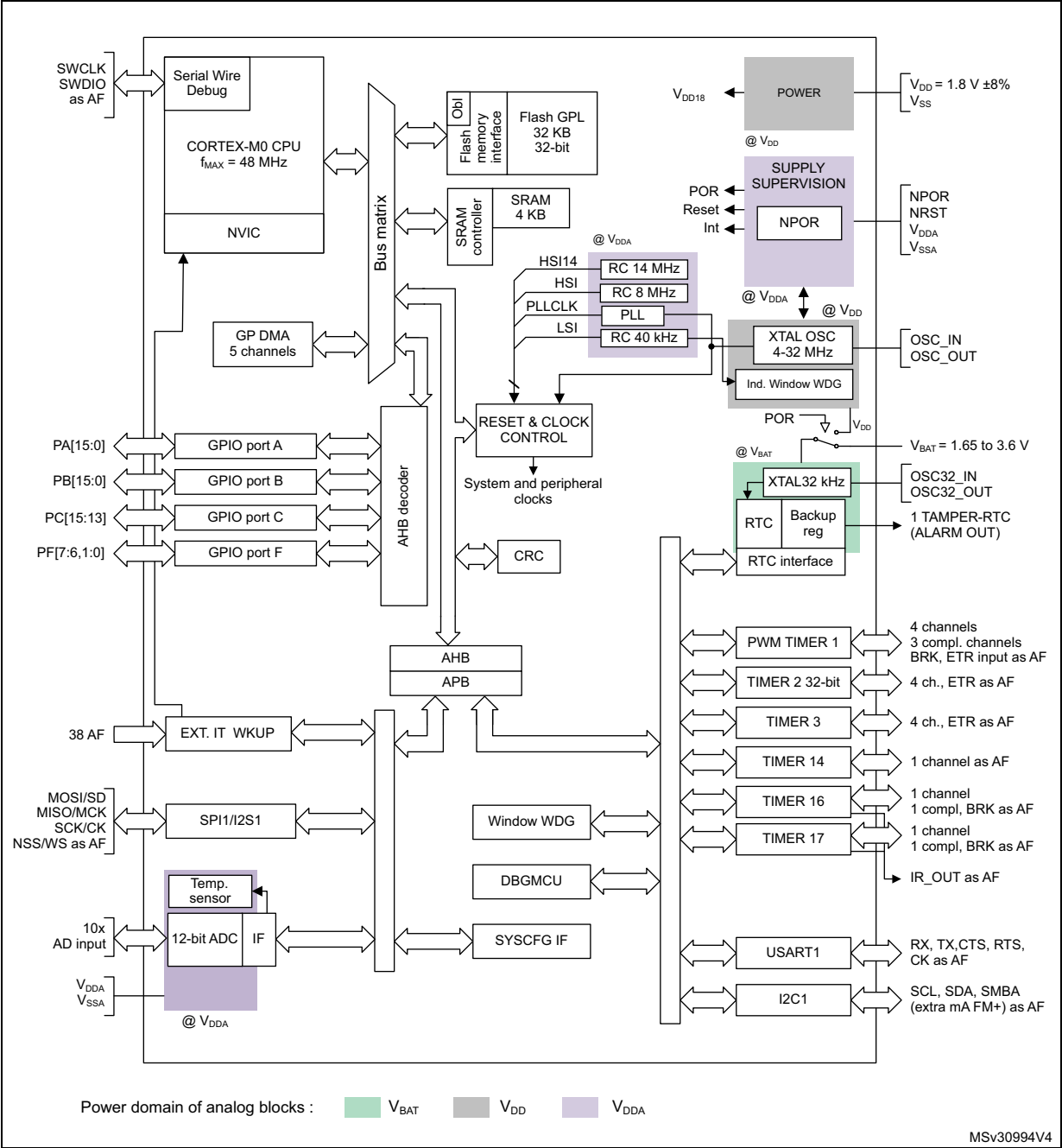
Figure 1. Block diagram
