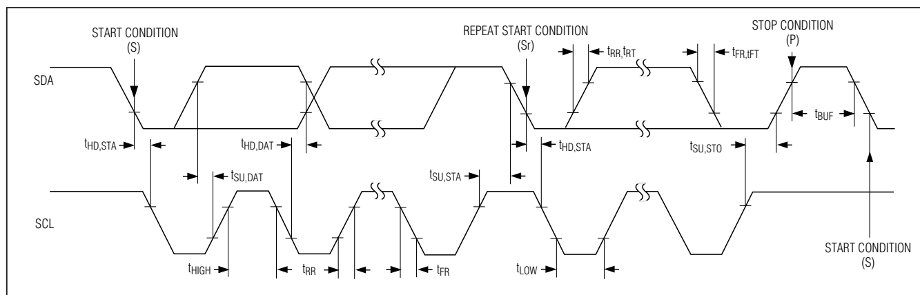
Figure 1. I 2 C Serial-Interface Timing
