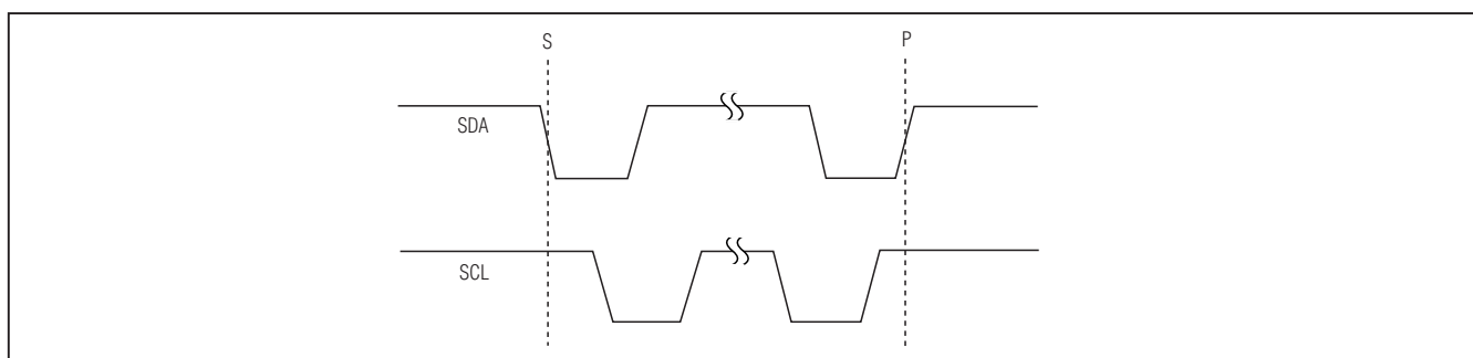
Figure 7. START and STOP Conditions
