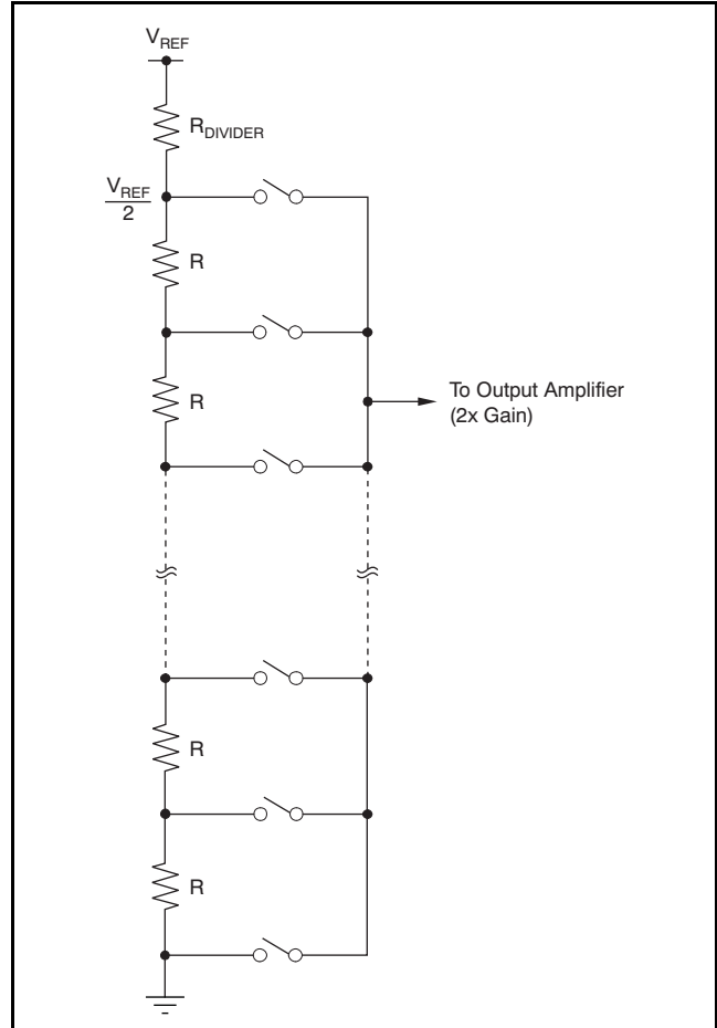
Figure 93. Resistor String
