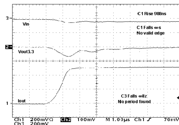
Figure 24 : Load Transient
