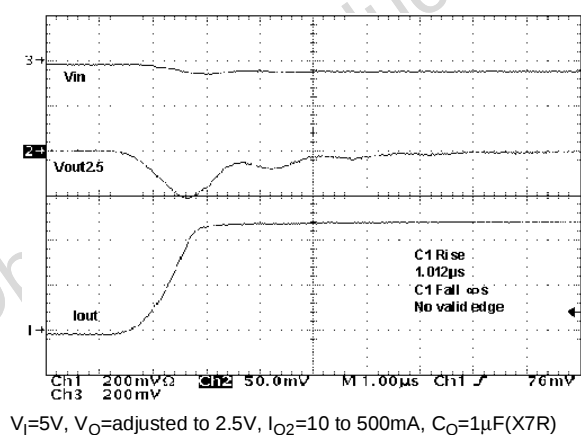
Figure 23 : Load Transient
