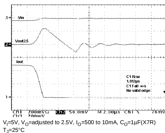
Figure 23 : Load Transient
