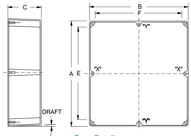
Base Detail
