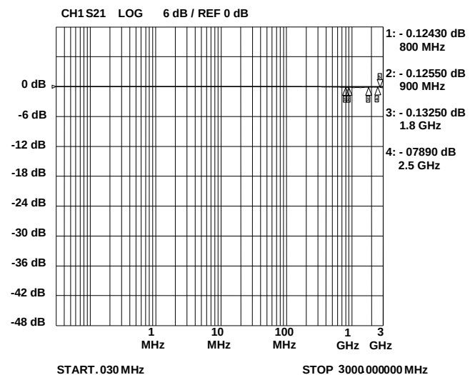
Insertion Loss
