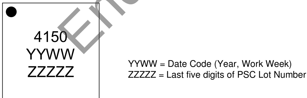
Figure 16. Marking Specification
