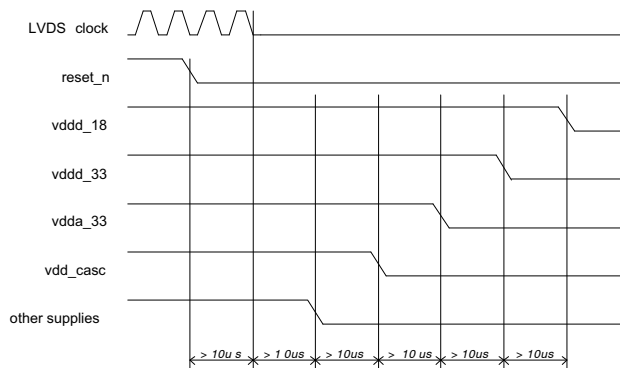
Figure 18. Power-down Sequence
