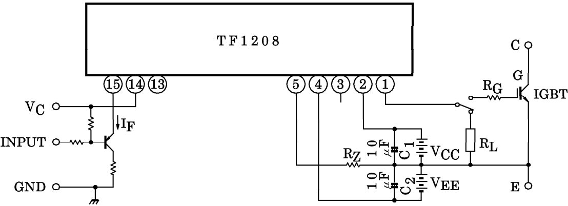
Fig.3 SWITCHING TIME TEST CIRCUIT
