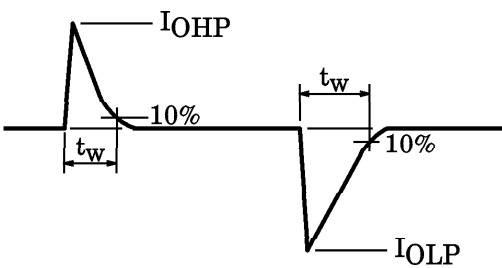
Fig.1 EXPONENTIAL WAVEFORM
