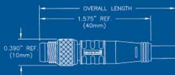
STRAIGHT FEMALE SINGLE ENDED THREADED COUPLING
