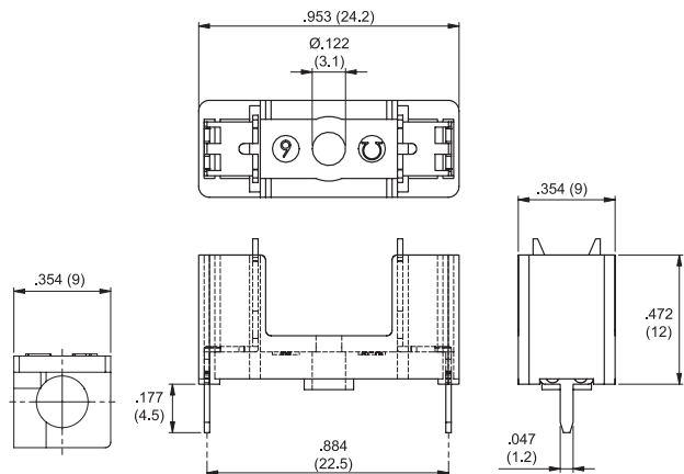
FH-320-NV Holder
