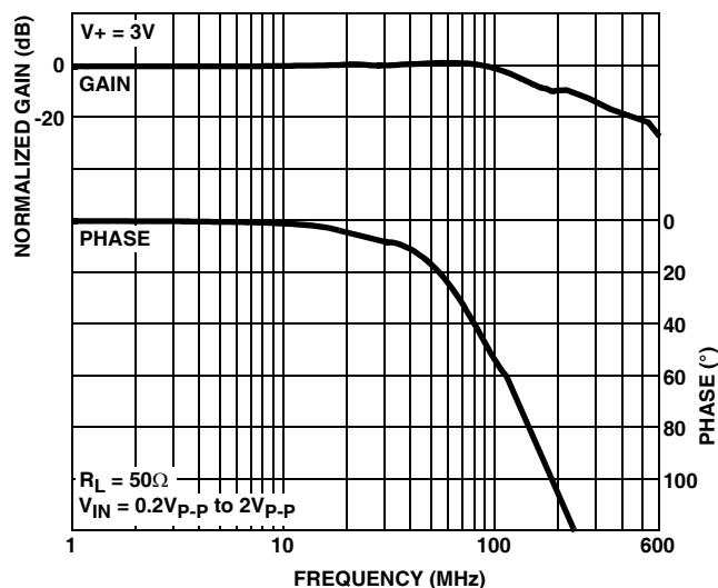
FIGURE 22. FREQUENCY RESPONSE
