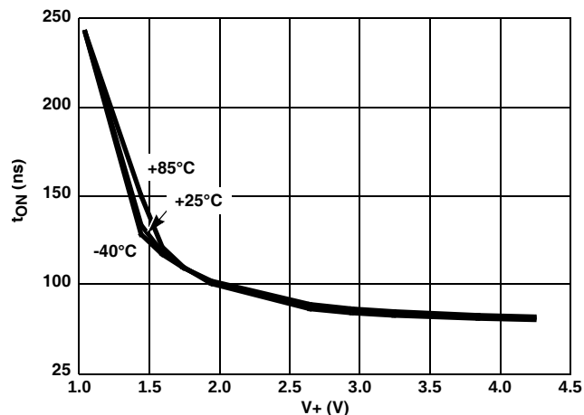
FIGURE 20. TURN-ON TIME vs SUPPLY VOLTAGE
