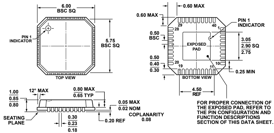
Figure 24. 40-Lead Lead Frame Chip Scale Package [LFCSP_VQ] 6 mm x 6 mm Body, Very Thin Quad (CP-40-8) Dimensions shown in millimeters
