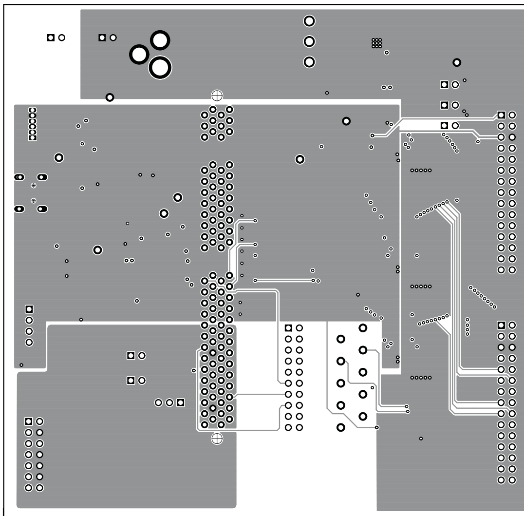
Figure 20. HPA358A Layer 3
