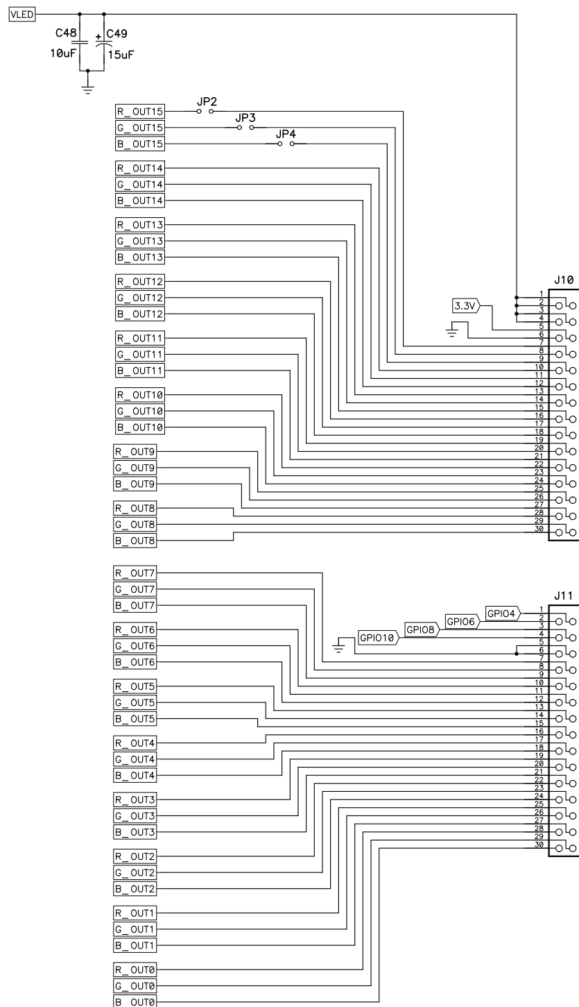
Figure 11. HPA358A Schematic 5
