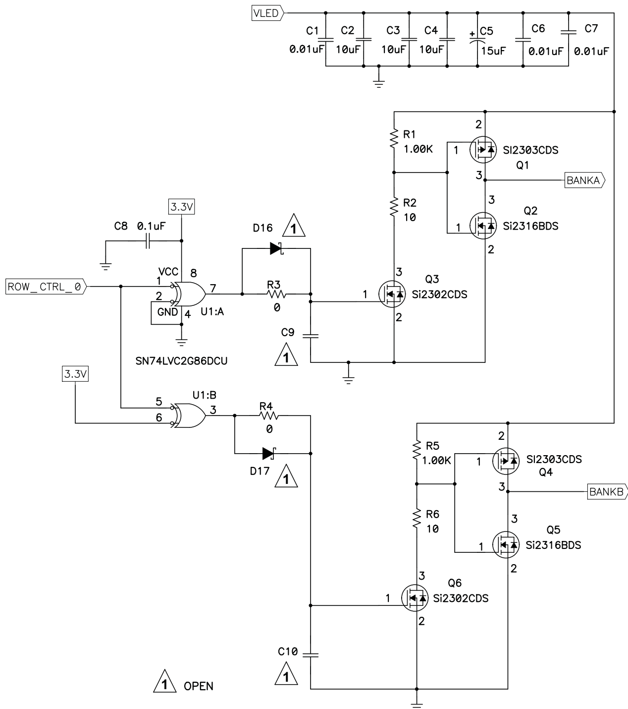
Figure 6. HPA357A - Schematic 2
