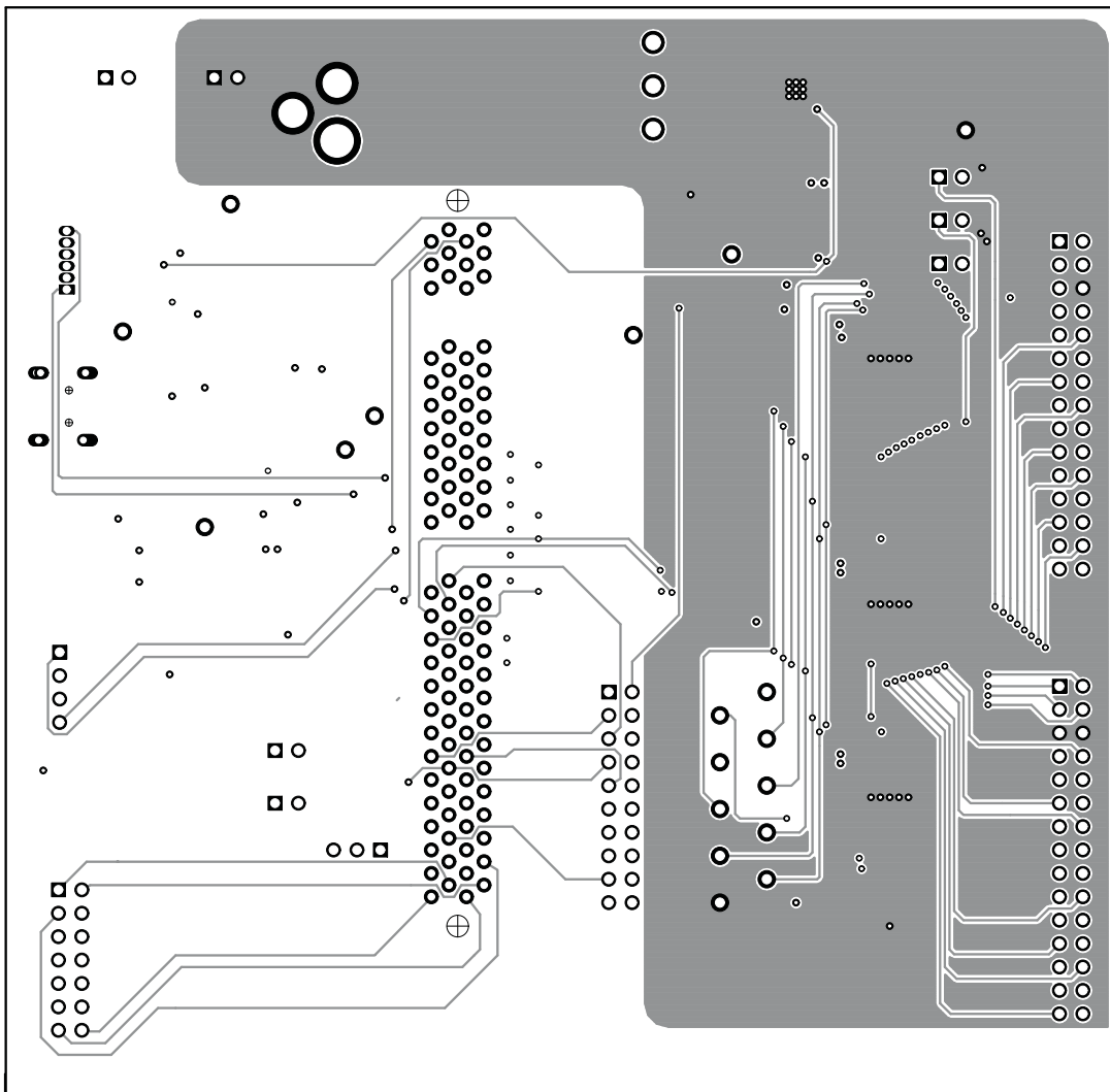
Figure 19. HPA358A Layer 2
