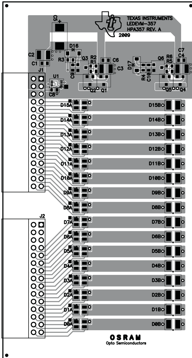
Figure 12. HPA357A Assembly Layer Routing
