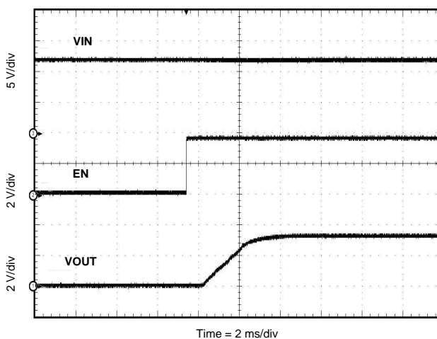
Figure 16. Start Up Relative to EN
