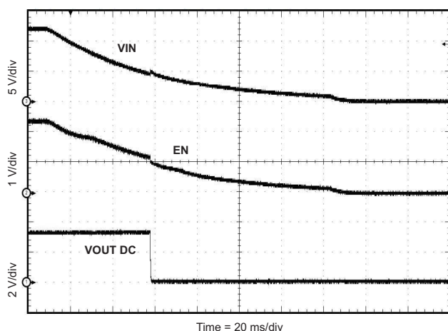
Figure 18. Shutdown Relative to V_{IN}
