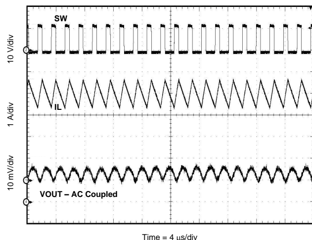
Figure 12. Output Voltage Ripple CCM
