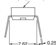
Flat Actuator With Seal Tape Seal tape (t = 0.06)
