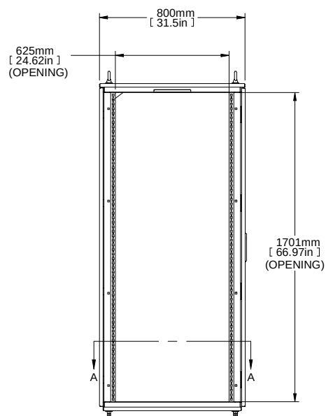
L.S. VIEW
