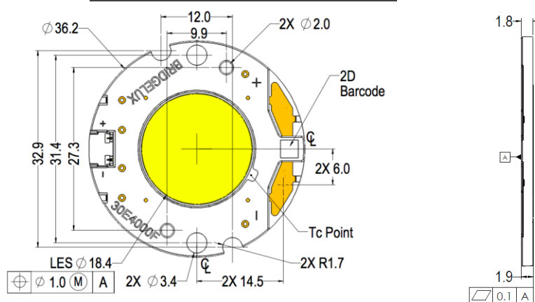
Figure 9: Drawing for Vero 18 LED Array
