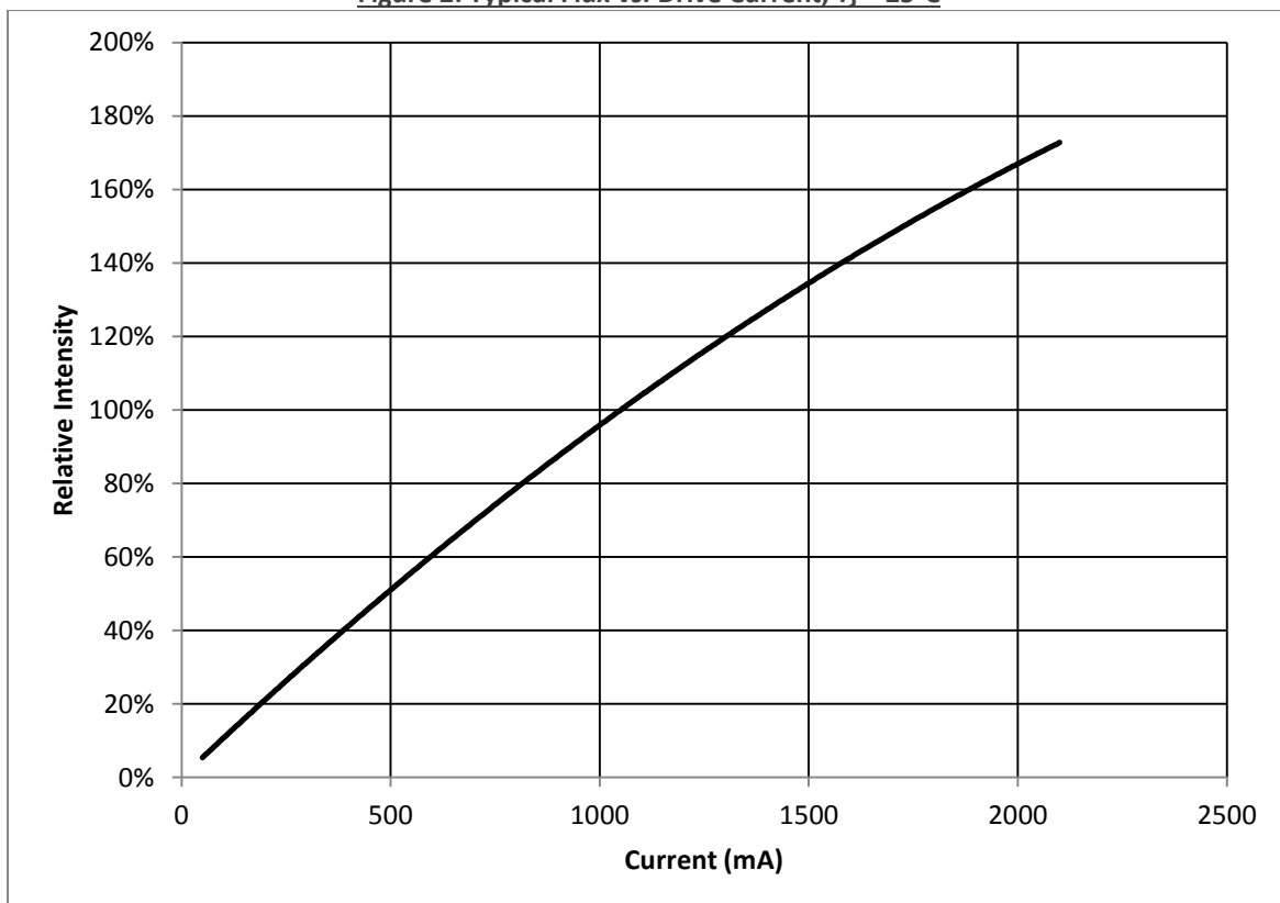
Figure 2: Typical Flux vs. Drive Current, Tj = 25°C
