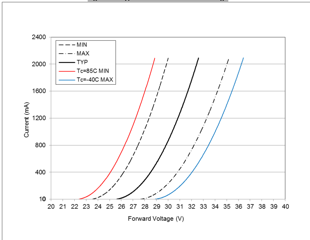
Figure 1: Typical Drive Current vs. Voltage
