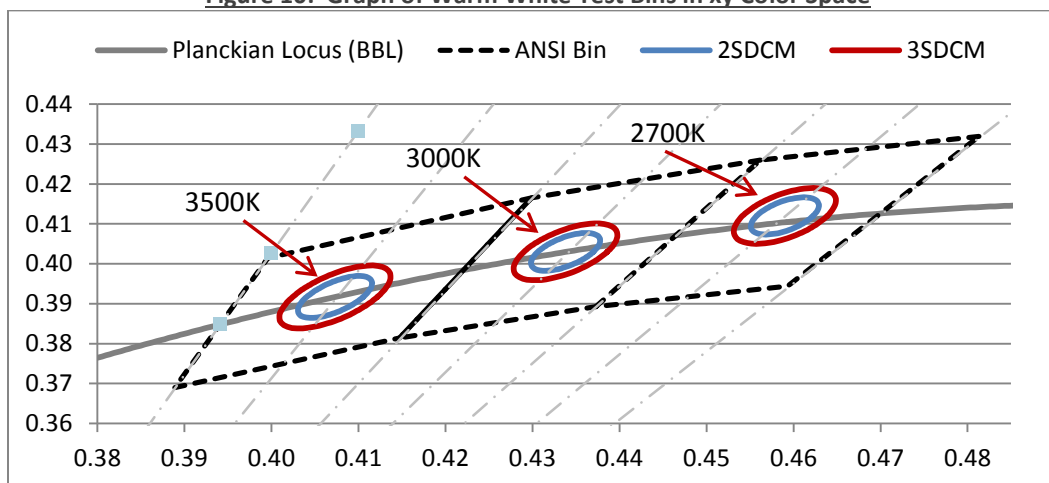
Figure 10: Graph of Warm White Test Bins in xy Color Space
