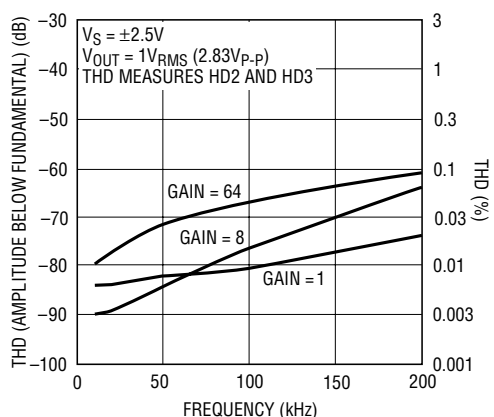
LTC6910-2 Distortion with Light Loading ( R_L = 10k )
