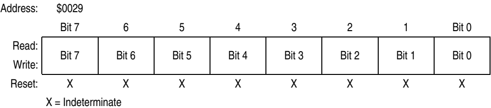
Figure 12-36. PWM Counter Modulo Register Low (PMODL)
