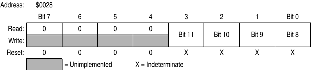
Figure 12-35. PWM Counter Modulo Register High (PMODH)
