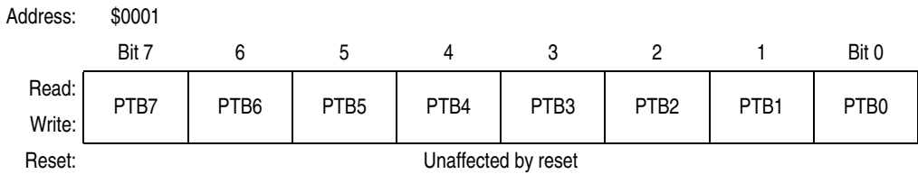
Figure 10-5. Port B Data Register (PTB)
