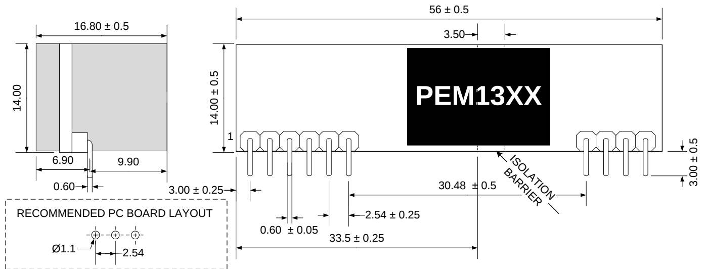
Figure 6 – PHYSICAL PACKAGE
