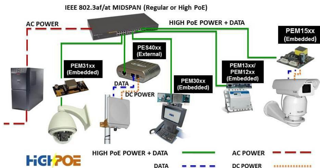
Figure 9 – Sample PoE System Configuration
