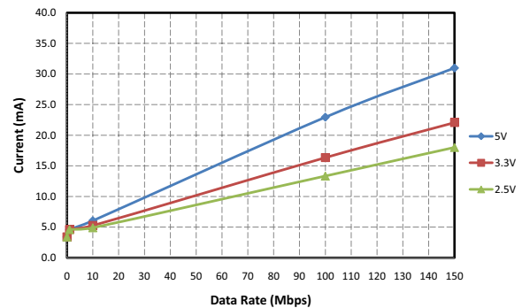
Figure 13. Si8661 Typical V_{DD2} Supply Current vs. Data Rate 5, 3.3, and 2.5 V Operation (15 pF Load)
