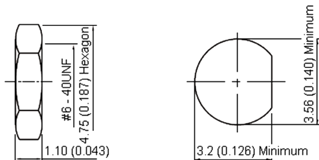
Mounting Hole
