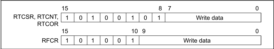
Figure 12.4 Writing to RFCR, RTCSR, RTCNT, and RTCOR
