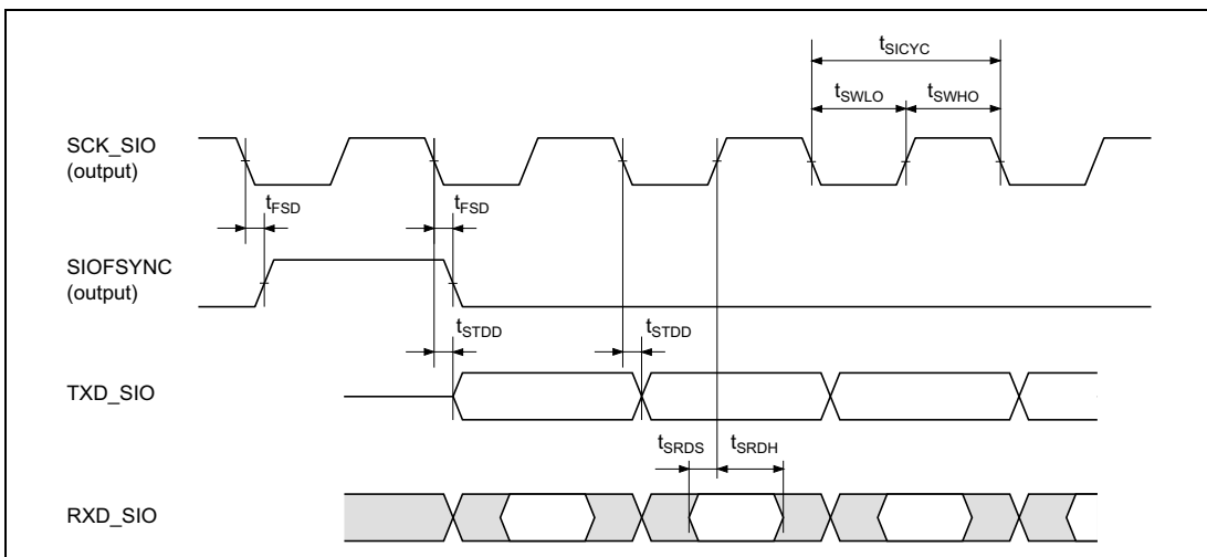
Figure 32.52 SIOF Transmit/Receive Timing (Master Mode 1: Rise Sampling Time)
