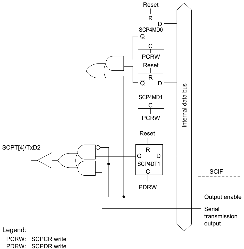
Figure 19.2 SCPT[4]/TxD2 Pin
