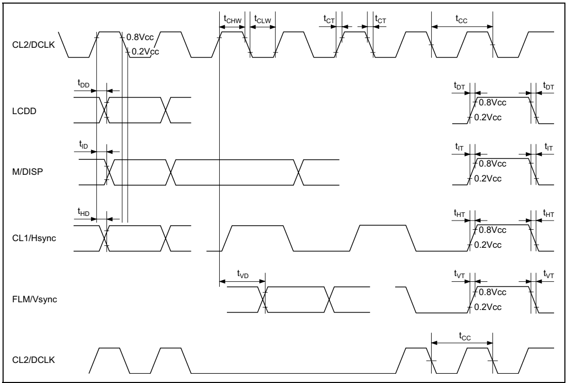
Figure 32.49 LCDC AC Specification
