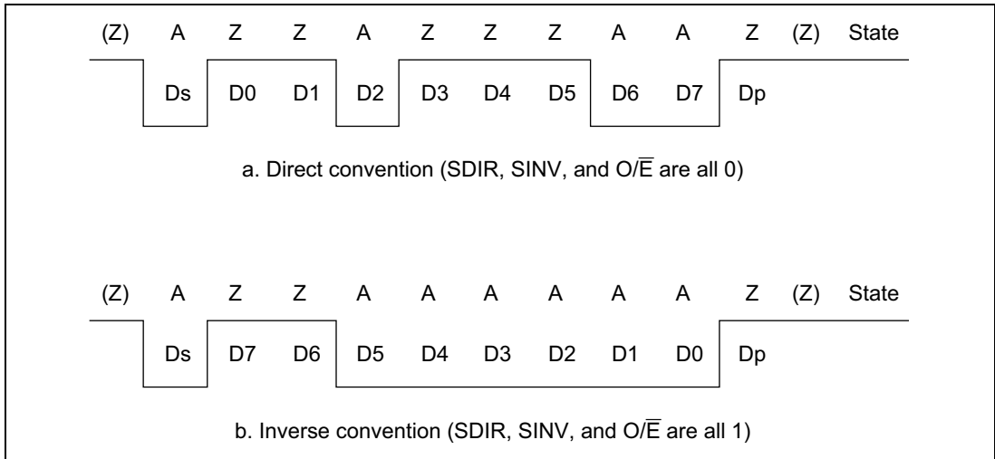
Figure 18.4 Waveform of Start Character
