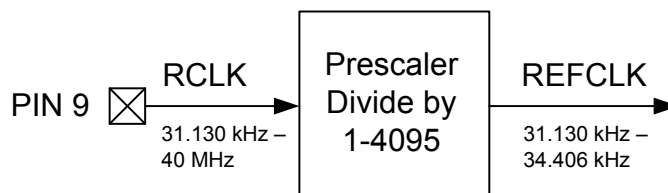
Figure 2. REFCLK Prescaler
