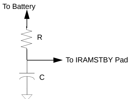
Figure 2. Recommended Connection Diagram for IRAMSTBY
