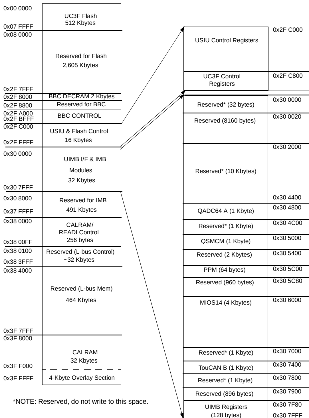
Figure 4. MPC533 Internal Memory Map
