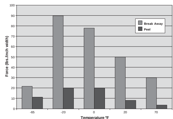
Figure 1. T-Peel Performance vs. Temperature (3M™ VHB™ Adhesive Transfer Tape F9473PC on Aluminum)
