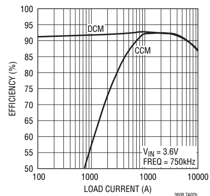
Efficiency Curve
