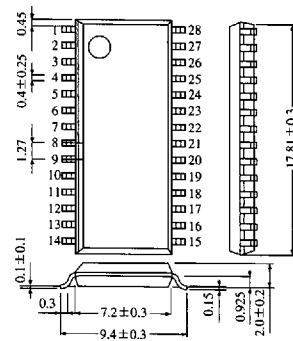
28-Pin PANAFLAT Package (SO-28D) (SOP028-P-0375A)
