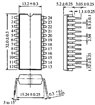
24-Pin DIL Plastic Package (DIP024-P-0600B)
