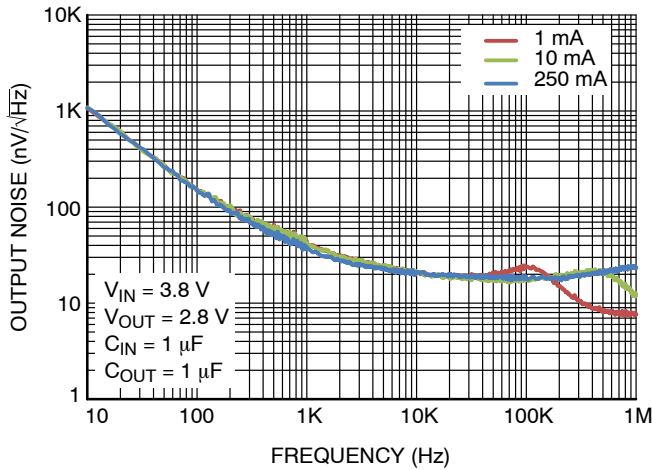
Figure 28. Output Voltage Noise Spectral Density – V_{\text{OUT}} = 2.8 \text{ V}
