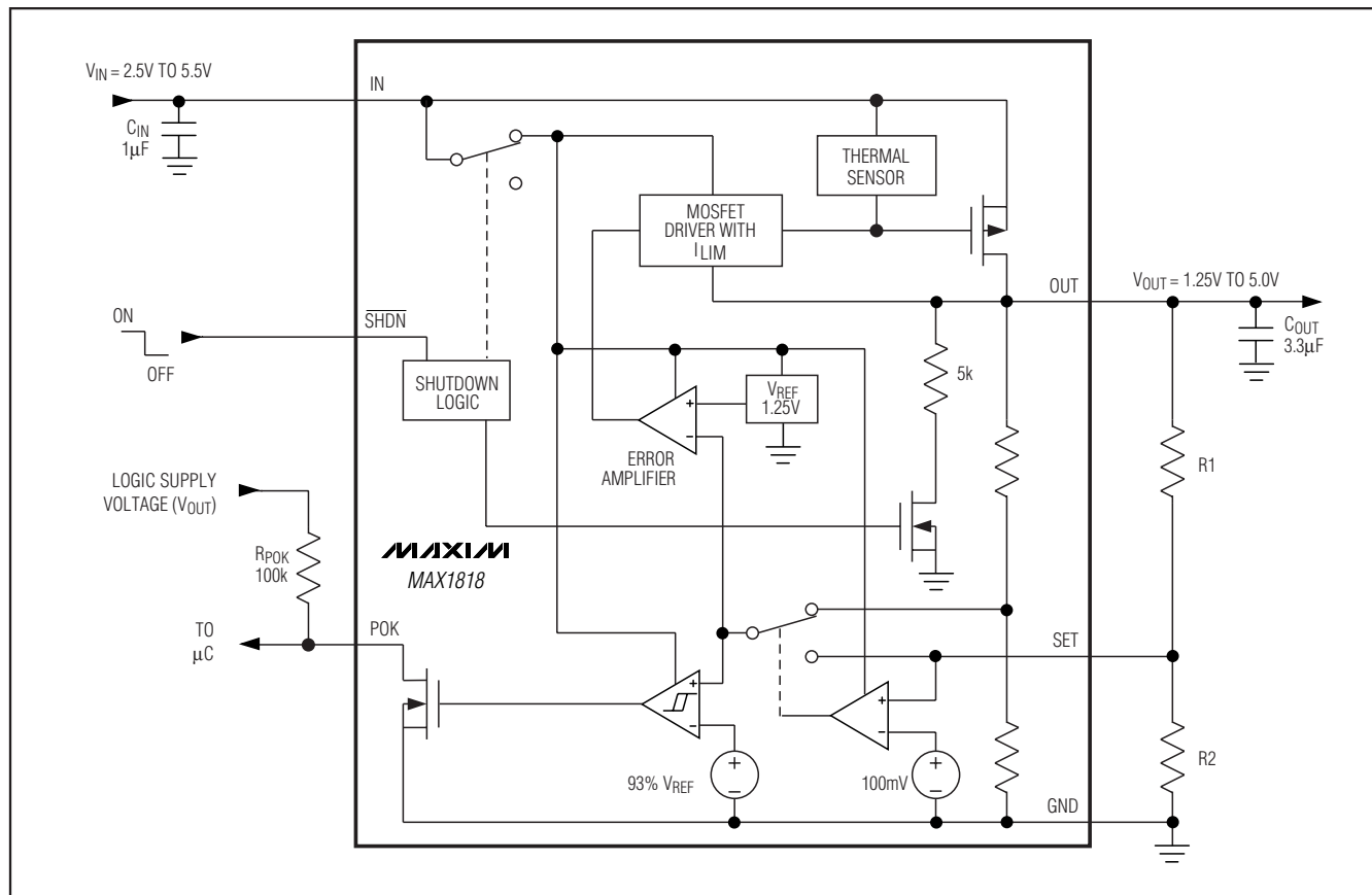
Figure 1. Functional Diagram
