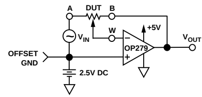
Figure 33. Inverting Programmable Gain Test Circuit
