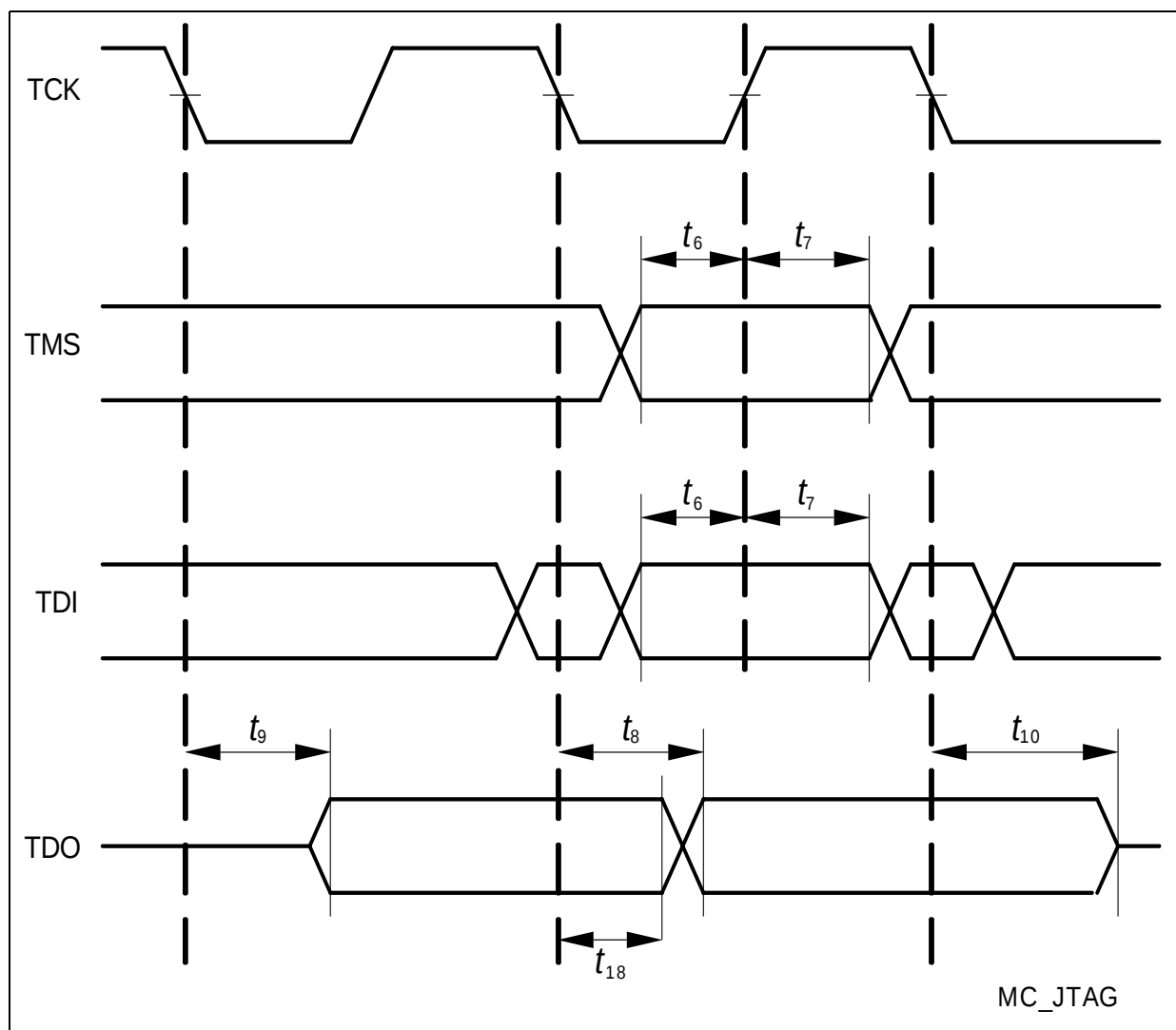
Figure 29 JTAG Timing
