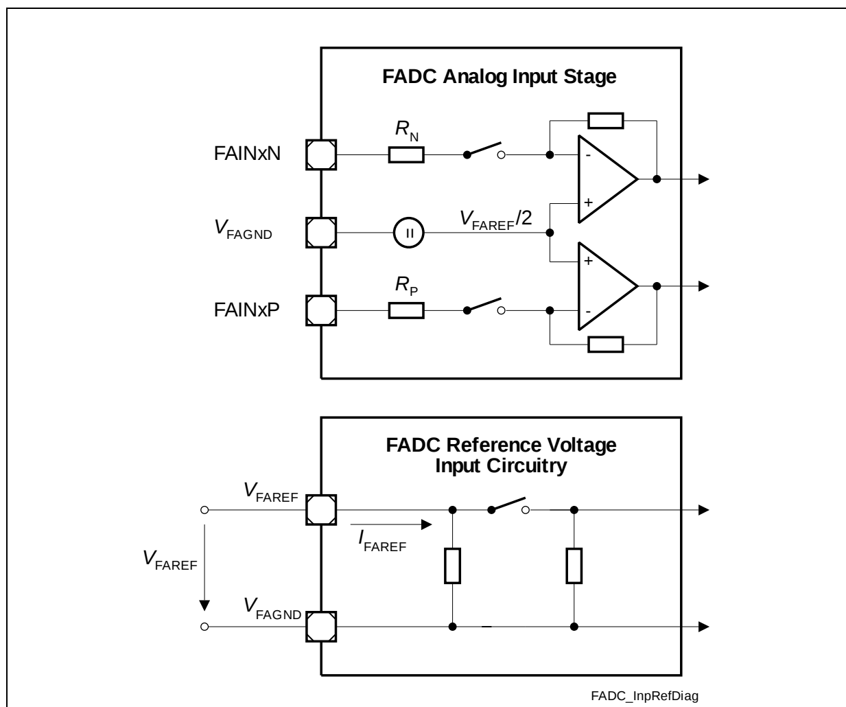
Figure 20 FADC Input Circuits
