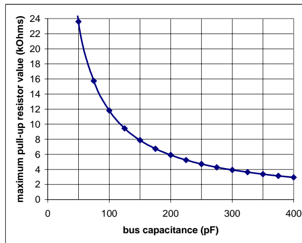
Figure 9. Max pull-up resistor value (standard mode)
