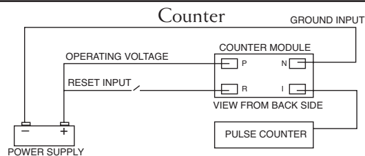
C1141AB Counter
