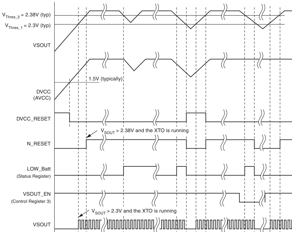
Figure 5-3. Reset Timing
