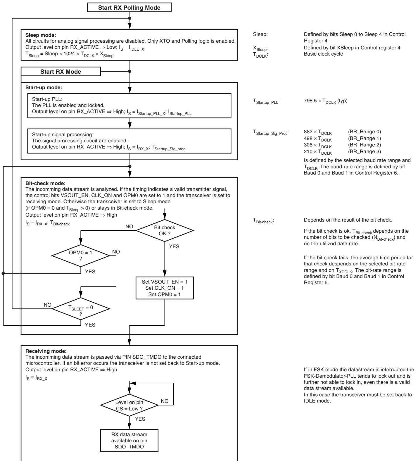
Figure 9-2. Flow Chart Polling Mode/RX Mode ( T_{\text{MODE}} = 1 , Transparent Mode Active)
