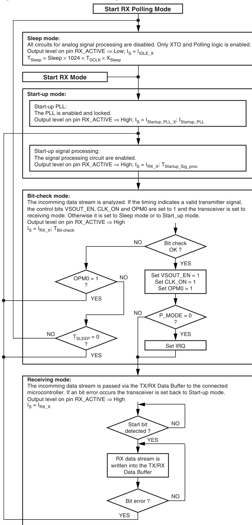
Figure 9-1. Flow Chart Polling Mode/RX Mode ( T_{\text{MODE}} = 0 , Transparent Mode Inactive)
