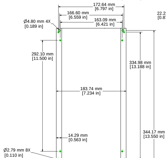
TOP PANEL - BOTTOM VIEW
