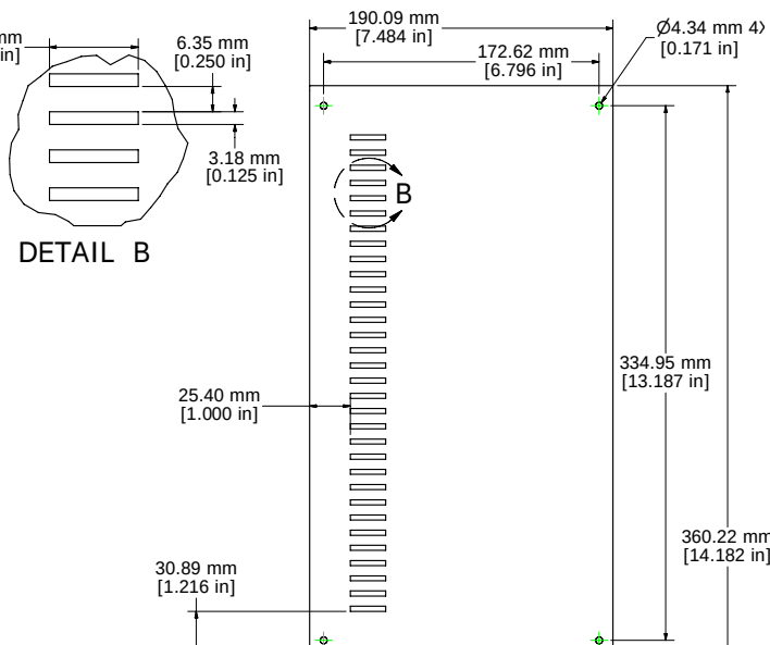
ENCLOSURE CASE - BOTTOM VIEW
