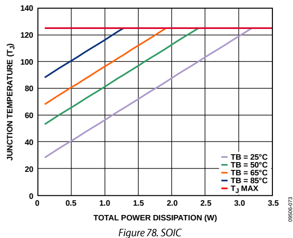
Figure 78. SOIC
