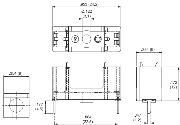
FH-320-NV Holder
