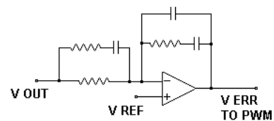
FIGURE 15. TYPICAL ANALOG ERROR AMPLIFIER AND COMPENSATION
