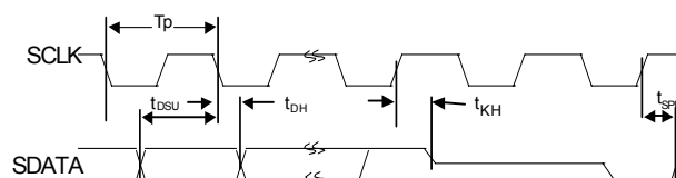
FIGURE 6. ISL6590 DATA WRITE TIMING
