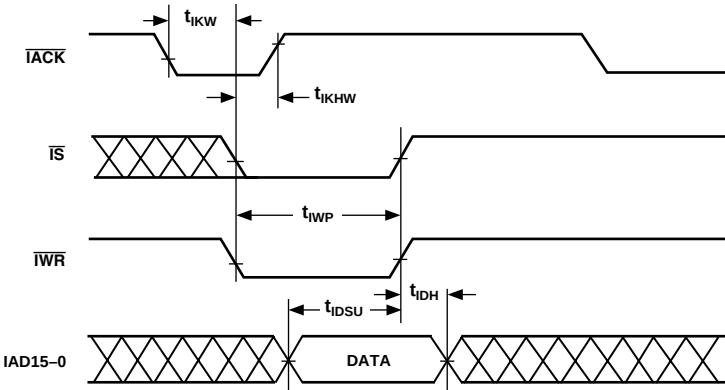
Figure 27. IDMA Write, Short Write Cycle
