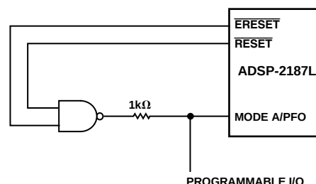
Figure 10. Mode A Pin/EZ-ICE Circuit
