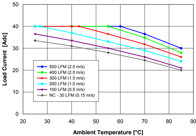
Fig. 3.3V.1: Available load current vs. ambient air temperature and airflow rates for QM48T40033 converter with B height pins mounted vertically with air flowing from pin 3 to pin 1, MOSFET temperature \leq 120^\circ\text{C} , V_{in} = 48\text{ V} .
