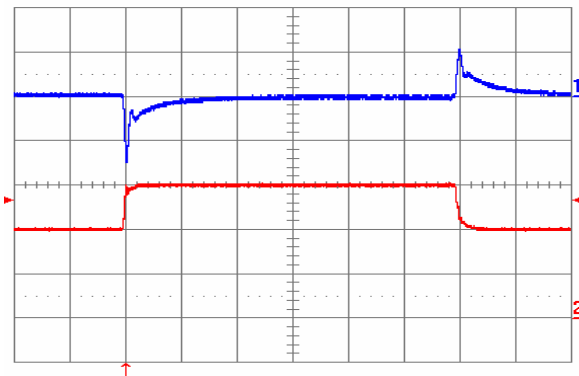
Fig. 1.8V.9: Output voltage response to load current step-change (20 A – 30 A – 20 A) at V_{in} = 48\text{ V} . Top trace: output voltage (100 mV/div.). Bottom trace: load current (10 A/div.). Current slew rate: 1 A/ \mu\text{s} . C_o = 470\text{ }\mu\text{F} tantalum + 1 \mu\text{F} ceramic. Time scale: 0.2 ms/div.
