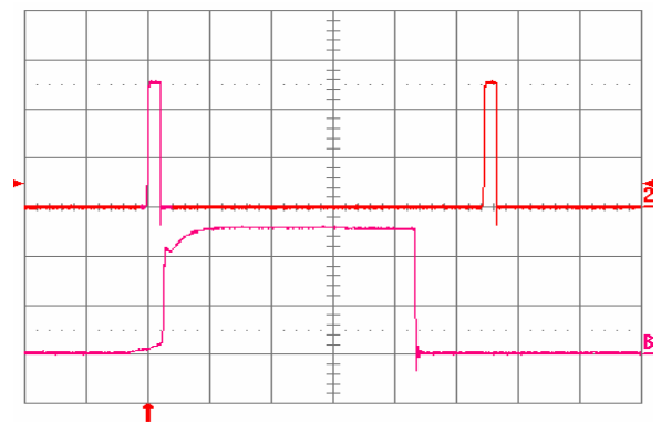
Fig. 1.5V.15: Load current (top trace, 20 A/div, 20 ms/div) into a 10 mΩ short circuit during restart, at V_{in} = 48 V. Bottom trace (20 A/div, 1 ms/div) is an expansion of the on-time portion of the top trace.
