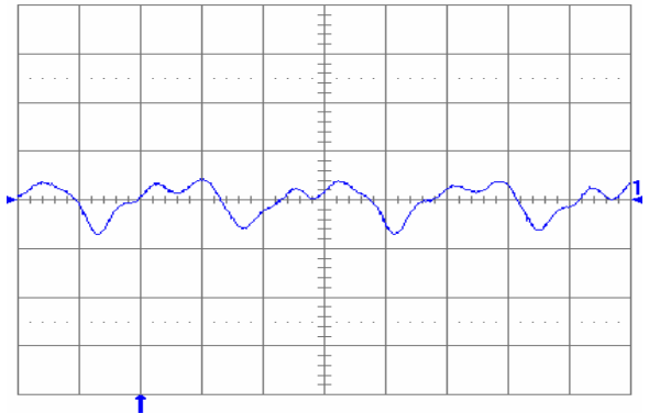
Fig. 1.8V.10: Output voltage ripple (20 mV/div.) at full rated load current into a resistive load with C_o = 10\text{ }\mu\text{F} tantalum + 1 \mu\text{F} ceramic and V_{in} = 48\text{ V} . Time scale: 1 \mu\text{s} /div.
