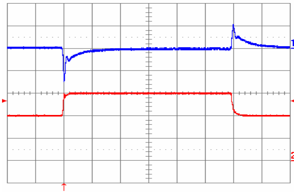
Fig. 1.5V.9: Output voltage response to load current step-change (20 A – 30 A – 20 A) at V_{in} = 48 V. Top trace: output voltage (100 mV/div.). Bottom trace: load current (10 A/div). Current slew rate: 1 A/ \mu s. C_o = 470 \mu F tantalum + 1 \mu F ceramic. Time scale: 0.2 ms/div.
