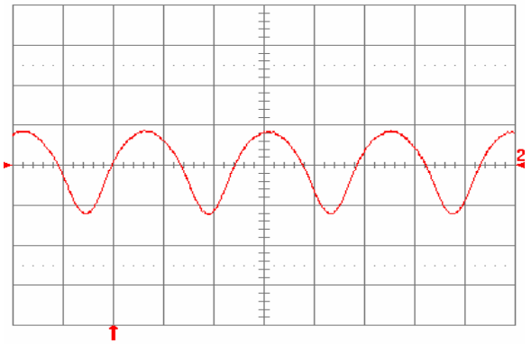
Fig. 1.2V.13: Input reflected ripple current, i_c (100 mA/div), measured at input terminals at full rated load current and V_{in} = 48 V. Refer to Fig. 1.2V.11 for test setup. Time scale: 1 µs/div.
