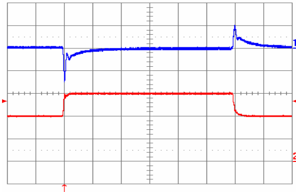
Fig. 2.0V.9: Output voltage response to load current step-change (20 A – 30 A – 20 A) at V_{in} = 48 V. Top trace: output voltage (100 mV/div.). Bottom trace: load current (10 A/div.). Current slew rate: 1 A/ \mu s. C_o = 470 \mu F tantalum + 1 \mu F ceramic. Time scale: 0.2 ms/div.
