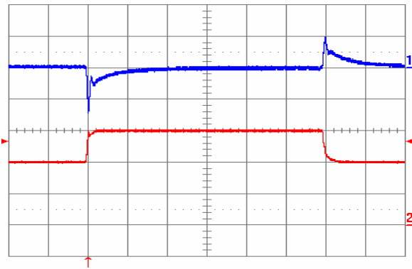
Fig. 3.3V.9: Output voltage response to load current step-change (20 A – 30 A – 20 A) at V_{in} = 48 V. Top trace: output voltage (100 mV/div.). Bottom trace: load current (10 A/div.). Current slew rate: 1 A/ \mu s. C_o = 470 \mu F tantalum + 1 \mu F ceramic. Time scale: 0.2 ms/div.
