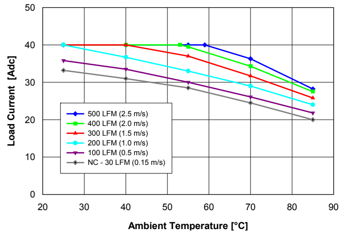
Fig. 3.3V.2: Available load current vs. ambient air temperature and airflow rates for QM48T40033 converter with B height pins mounted horizontally with air flowing from pin 3 to pin 1, MOSFET temperature \leq 120^\circ\text{C} , V_{in} = 48\text{ V} .
