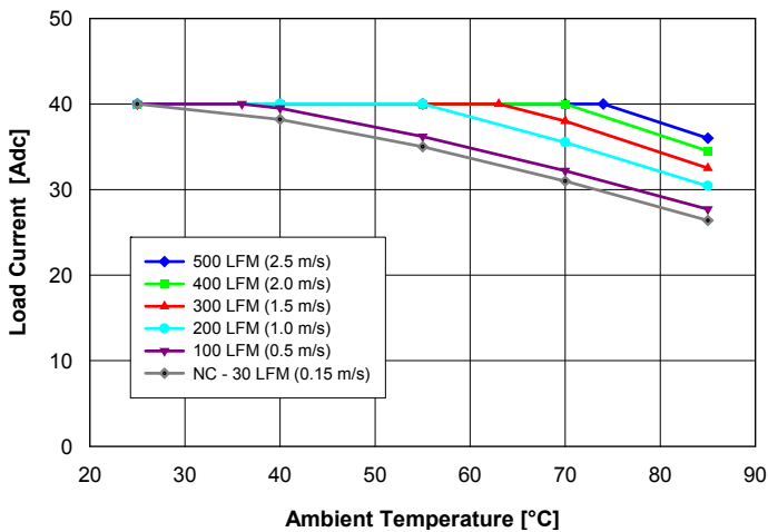
Fig. 1.5V.1: Available load current vs. ambient air temperature and airflow rates for QM48T40015 converter with B height pins mounted vertically with air flowing from pin 3 to pin 1, MOSFET temperature \leq 120^\circ\text{C} , V_{in} = 48\text{ V} .
