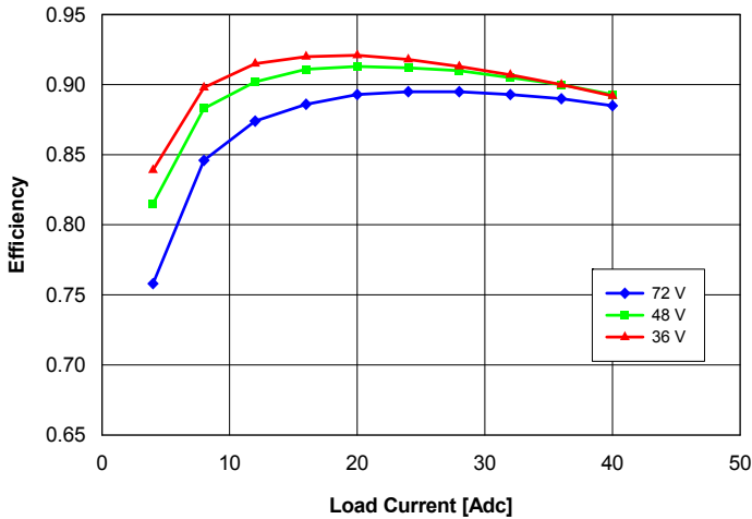
Fig. 2.5V.3: Efficiency vs. load current and input voltage for converter mounted vertically with air flowing from pin 3 to pin 1 at a rate of 300 LFM (1.5 m/s) and T_a = 25\text{ }^{\circ}\text{C} .
