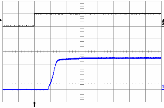
Fig. 2.5V.7: Turn-on transient at full rated load current (resistive) with no output capacitor at V_{in} = 48 V, triggered via ON/OFF pin. Top trace: ON/OFF signal (5 V/div.). Bottom trace: output voltage (1 V/div.) Time scale: 2 ms/div.
