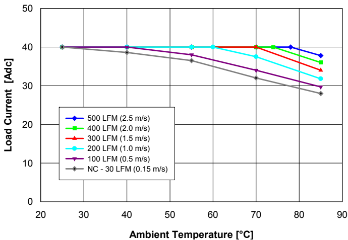
Fig. 1.0V.1: Available load current vs. ambient air temperature and airflow rates for QM48T40010 converter with B height pins mounted vertically with air flowing from pin 3 to pin 1, MOSFET temperature \leq 120^\circ\text{C} , V_{in} = 48\text{ V} .
