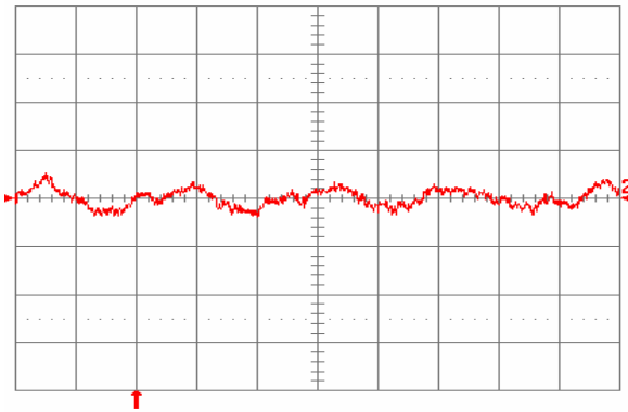
Fig. 1.8V.12: Input reflected ripple current, i_s (10 mA/div), measured through 10\ \mu\text{H} at the source at full rated load current and V_{in} = 48\ \text{V} . Refer to Fig. 1.8V.11 for test setup. Time scale: 1 \mu\text{s}/\text{div} .
