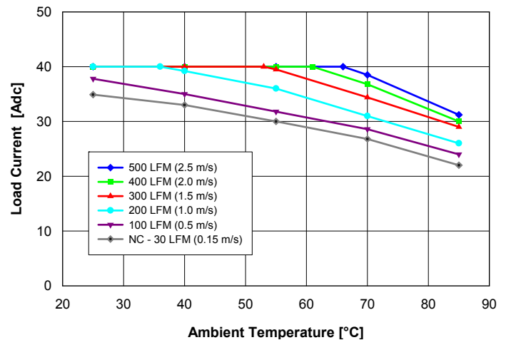
Fig. 2.5V.2: Available load current vs. ambient air temperature and airflow rates for QM48T40025 converter with B height pins mounted horizontally with air flowing from pin 3 to pin 1, MOSFET temperature \leq 120^\circ\text{C} , V_{in} = 48\text{ V} .
