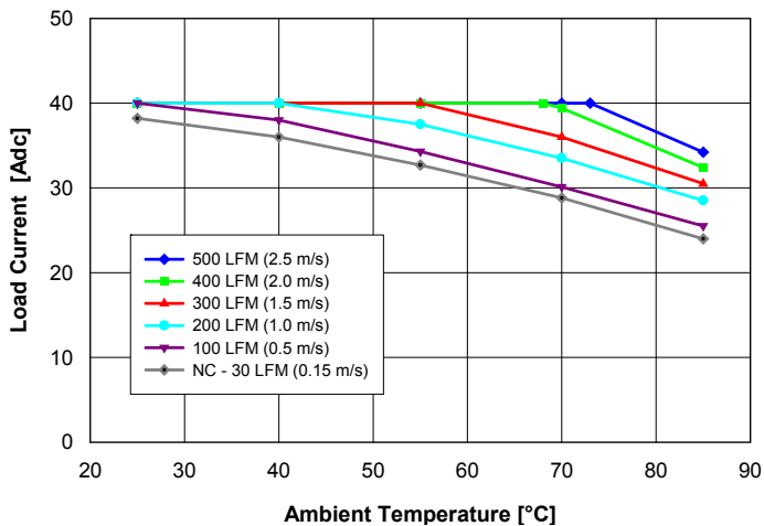
Fig. 2.0V.1: Available load current vs. ambient air temperature and airflow rates for QM48T40020 converter with B height pins mounted vertically with air flowing from pin 3 to pin 1, MOSFET temperature \leq 120^\circ\text{C} , V_{in} = 48\text{ V} .
