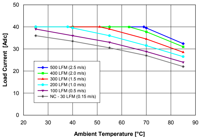
Fig. 2.5V.1: Available load current vs. ambient air temperature and airflow rates for QM48T40025 converter with B height pins mounted vertically with air flowing from pin 3 to pin 1, MOSFET temperature \leq 120^\circ\text{C} , V_{in} = 48\text{ V} .
