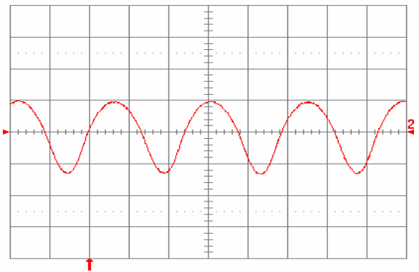
Fig. 1.5V.13: Input reflected ripple current, i_c (100 mA/div), measured at input terminals at full rated load current and V_{in} = 48 V. Refer to Fig. 1.5V.11 for test setup. Time scale: 1 µs/div.
