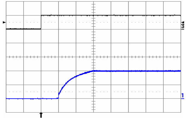
Fig. 2.0V.8: Turn-on transient at full rated load current (resistive) plus 40,000 \mu F at V_{in} = 48 V, triggered via ON/OFF pin. Top trace: ON/OFF signal (5 V/div.). Bottom trace: output voltage (1 V/div.). Time scale: 2 ms/div.
