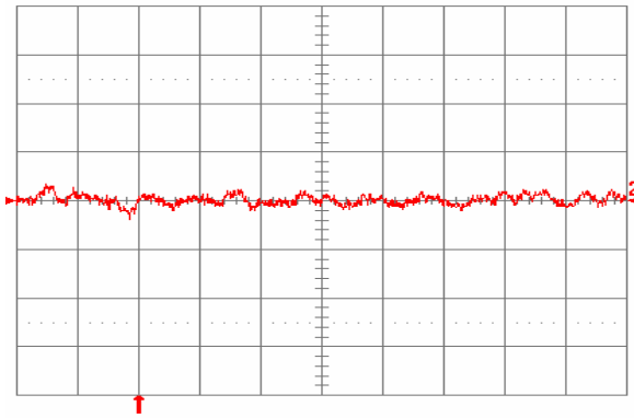
Fig. 1.2V.12: Input reflected ripple current, i_s (10 mA/div), measured through 10 µH at the source at full rated load current and V_{in} = 48 V. Refer to Fig. 1.2V.11 for test setup. Time scale: 1 µs/div.
