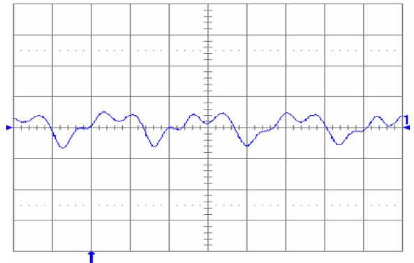
Fig. 2.0V.10: Output voltage ripple (20 mV/div.) at full rated load current into a resistive load with C_o = 10 \mu F tantalum + 1 \mu F ceramic and V_{in} = 48 V. Time scale: 1 \mu s/div.
