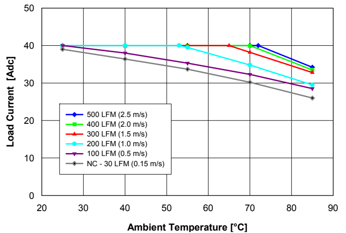
Fig. 1.5V.2: Available load current vs. ambient air temperature and airflow rates for QM48T40015 converter with B height pins mounted horizontally with air flowing from pin 3 to pin 1, MOSFET temperature \leq 120^\circ\text{C} , V_{in} = 48\text{ V} .
