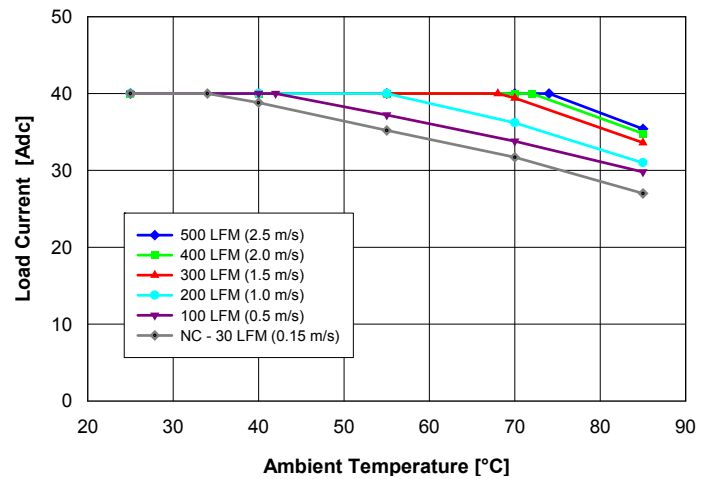
Fig. 1.2V.2: Available load current vs. ambient air temperature and airflow rates for QM48T40012 converter with B height pins mounted horizontally with air flowing from pin 3 to pin 1, MOSFET temperature \leq 120^\circ\text{C} , V_{in} = 48\text{ V} .
