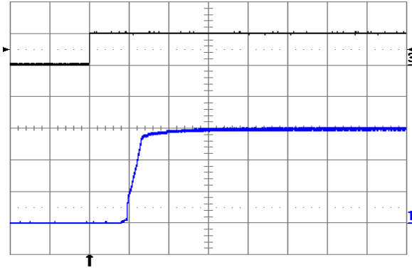
Fig. 1.5V.7: Turn-on transient at full rated load current (resistive) with no output capacitor at V_{in} = 48 V, triggered via ON/OFF pin. Top trace: ON/OFF signal (5 V/div.). Bottom trace: output voltage (0.5 V/div.) Time scale: 2 ms/div.
