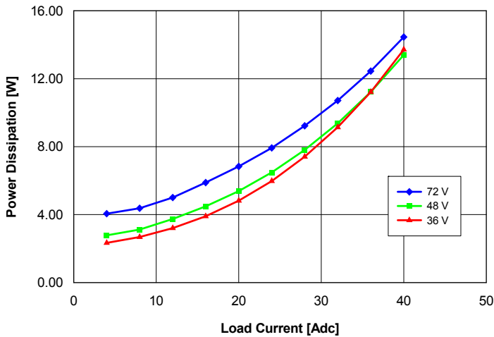
Fig. 3.3V.5: Power dissipation vs. load current and input voltage for converter mounted vertically with air flowing from pin 3 to pin 1 at a rate of 300 LFM (1.5 m/s) and T_a = 25\text{ }^{\circ}\text{C} .
