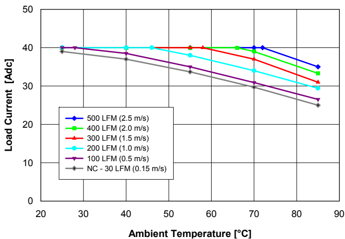
Fig. 1.8V.1: Available load current vs. ambient air temperature and airflow rates for QM48T40018 converter with B height pins mounted vertically with air flowing from pin 3 to pin 1, MOSFET temperature \leq 120^\circ\text{C} , V_{in} = 48\text{ V} .
