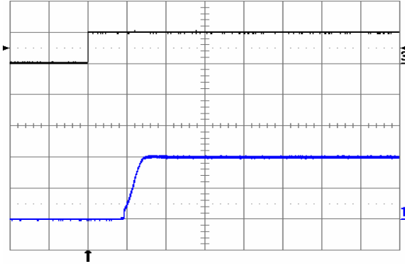
Fig. 2.0V.7: Turn-on transient at full rated load current (resistive) with no output capacitor at V_{in} = 48 V, triggered via ON/OFF pin. Top trace: ON/OFF signal (5 V/div.). Bottom trace: output voltage (1 V/div.). Time scale: 2 ms/div.
