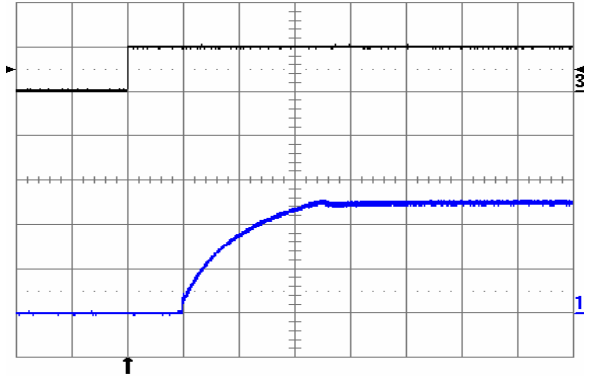
Fig. 2.5V.8: Turn-on transient at full rated load current (resistive) plus 40,000 \mu F at V_{in} = 48 V, triggered via ON/OFF pin. Top trace: ON/OFF signal (5 V/div.). Bottom trace: output voltage (1 V/div.). Time scale: 2 ms/div.
