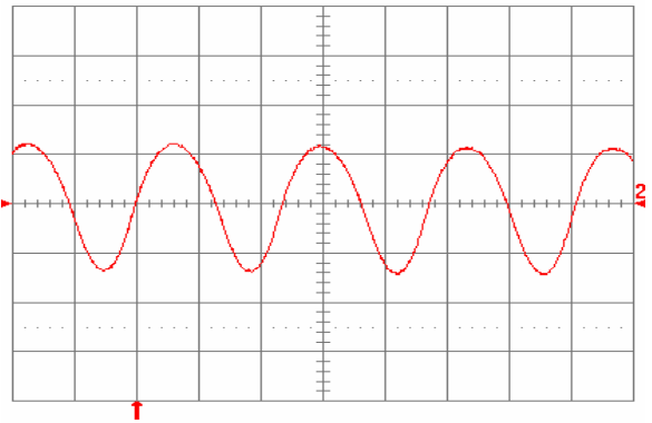
Fig. 1.8V.13: Input reflected ripple current, i_c (100 mA/div), measured at input terminals at full rated load current and V_{in} = 48\ \text{V} . Refer to Fig. 1.8V.11 for test setup. Time scale: 1 \mu\text{s}/\text{div} .
