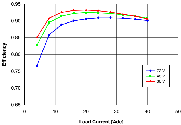
Fig. 3.3V.3: Efficiency vs. load current and input voltage for converter mounted vertically with air flowing from pin 3 to pin 1 at a rate of 300 LFM (1.5 m/s) and T_a = 25\text{ }^{\circ}\text{C} .
