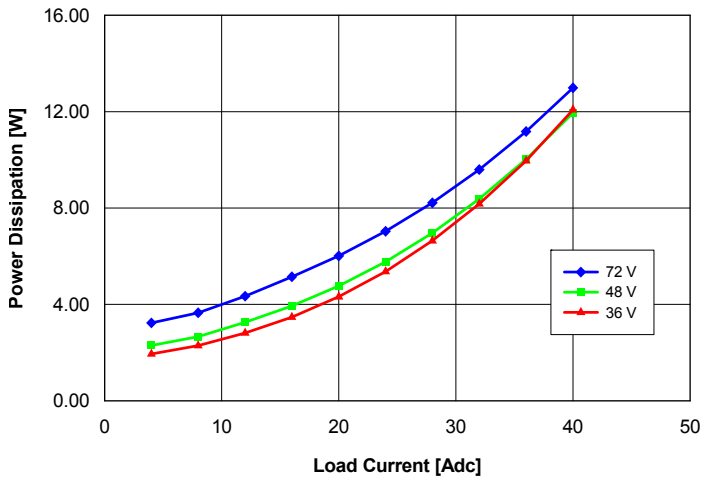
Fig. 2.5V.5: Power dissipation vs. load current and input voltage for converter mounted vertically with air flowing from pin 3 to pin 1 at a rate of 300 LFM (1.5 m/s) and T_a = 25\text{ }^{\circ}\text{C} .
