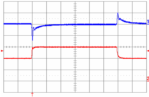
Fig. 2.5V.9: Output voltage response to load current step-change (20 A – 30 A – 20 A) at V_{in} = 48 V. Top trace: output voltage (100 mV/div.). Bottom trace: load current (10 A/div). Current slew rate: 1 A/ \mu s. C_o = 470 \mu F tantalum + 1 \mu F ceramic. Time scale: 0.2 ms/div.
