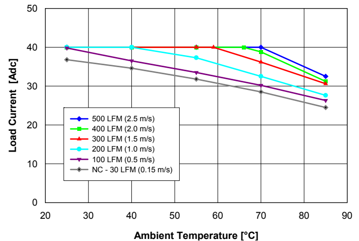
Fig. 2.0V.2: Available load current vs. ambient air temperature and airflow rates for QM48T40020 converter with B height pins mounted horizontally with air flowing from pin 3 to pin 1, MOSFET temperature \leq 120^\circ\text{C} , V_{in} = 48\text{ V} .
