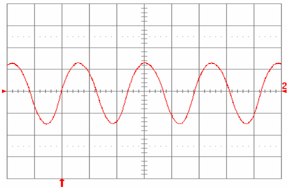
Fig. 2.0V.13: Input reflected ripple current, i_c (100 mA/div), measured at input terminals at full rated load current and V_{in} = 48 V. Refer to Fig. 2.0V.11 for test setup. Time scale: 1 µs/div.
