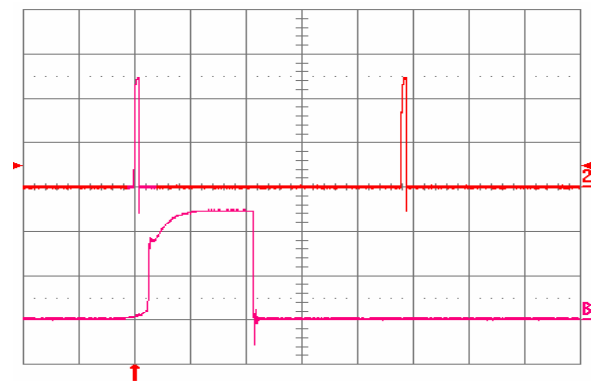
Fig. 2.5V.15: Load current (top trace, 20 A/div, 20 ms/div) into a 10 mΩ short circuit during restart, at V_{in} = 48 V. Bottom trace (20 A/div, 1 ms/div) is an expansion of the on-time portion of the top trace.
