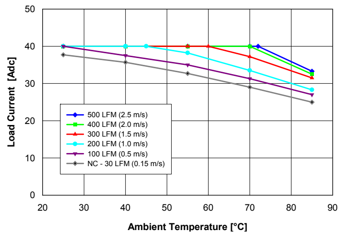
Fig. 1.8V.2: Available load current vs. ambient air temperature and airflow rates for QM48T40018 converter with B height pins mounted horizontally with air flowing from pin 3 to pin 1, MOSFET temperature \leq 120^\circ\text{C} , V_{in} = 48\text{ V} .
