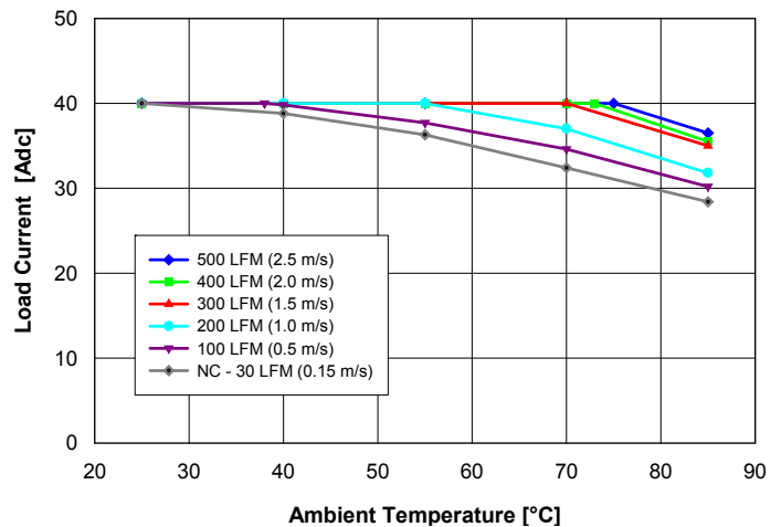
Fig. 1.0V.2: Available load current vs. ambient air temperature and airflow rates for QM48T40010 converter with B height pins mounted horizontally with air flowing from pin 3 to pin 1, MOSFET temperature \leq 120^\circ\text{C} , V_{in} = 48\text{ V} .
