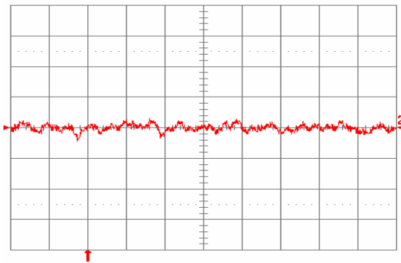
Fig. 1.0V.12: Input reflected ripple current, i_s (10 mA/div), measured through 10 μH at the source at full rated load current and V_{in} = 48 V. Refer to Fig. 1.0V.11 for test setup. Time scale: 1 μs/div.
