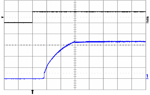
Fig. 1.8V.8: Turn-on transient at full rated load current (resistive) plus 40,000 \mu\text{F} at V_{in} = 48\text{ V} , triggered via ON/OFF pin. Top trace: ON/OFF signal (5 V/div.). Bottom trace: output voltage (1 V/div.). Time scale: 2 ms/div.
