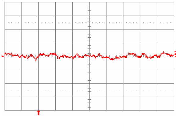
Fig. 2.0V.12: Input reflected ripple current, i_s (10 mA/div), measured through 10 µH at the source at full rated load current and V_{in} = 48 V. Refer to Fig. 2.0V.11 for test setup. Time scale: 1 µs/div.
