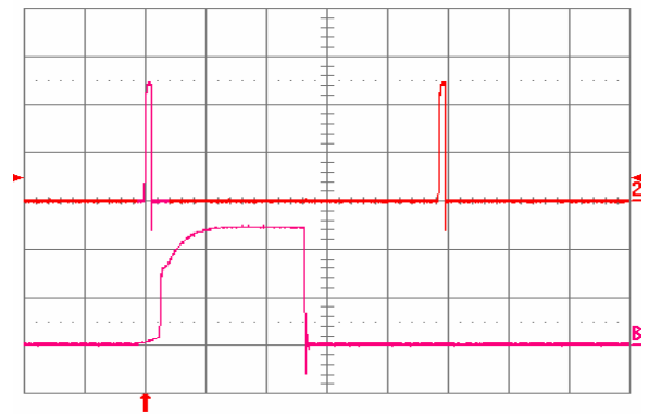
Fig. 2.0V.15: Load current (top trace, 20 A/div, 20 ms/div) into a 10 mΩ short circuit during restart, at V_{in} = 48 V. Bottom trace (20 A/div, 1 ms/div) is an expansion of the on-time portion of the top trace.
