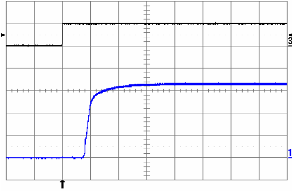
Fig. 3.3V.7: Turn-on transient at full rated load current (resistive) with no output capacitor at V_{in} = 48 V, triggered via ON/OFF pin. Top trace: ON/OFF signal (5 V/div.). Bottom trace: output voltage (1 V/div.). Time scale: 2 ms/div.
