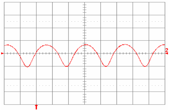
Fig. 1.0V.13: Input reflected ripple current, i_c (100 mA/div), measured at input terminals at full rated load current and V_{in} = 48 V. Refer to Fig. 1.0V.11 for test setup. Time scale: 1 μs/div.
