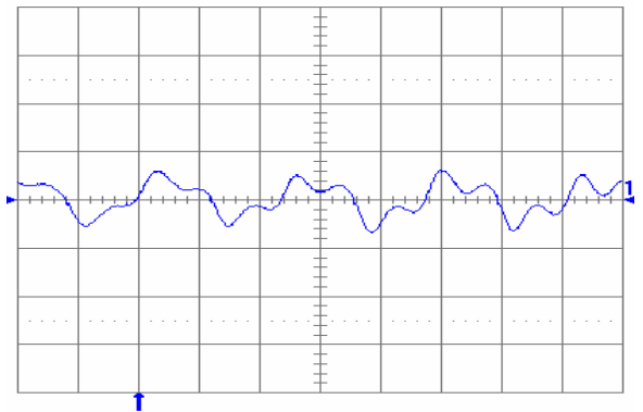
Fig. 2.5V.10: Output voltage ripple (20 mV/div.) at full rated load current into a resistive load with C_o = 10 \mu F tantalum + 1 \mu F ceramic and V_{in} = 48 V. Time scale: 1 \mu s/div.
