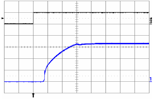
Fig. 3.3V.8: Turn-on transient at full rated load current (resistive) plus 40,000 \mu F at V_{in} = 48 V, triggered via ON/OFF pin. Top trace: ON/OFF signal (5 V/div.). Bottom trace: output voltage (1 V/div.). Time scale: 2 ms/div.
