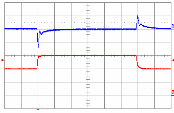
Fig. 1.0V.9: Output voltage response to load current step-change (20 A – 30 A – 20 A) at V_{in} = 48 V. Top trace: output voltage (100 mV/div.). Bottom trace: load current (10 A/div.). Current slew rate: 1 A/ \mu s. C_o = 470 \mu F tantalum + 1 \mu F ceramic. Time scale: 0.2 ms/div.
