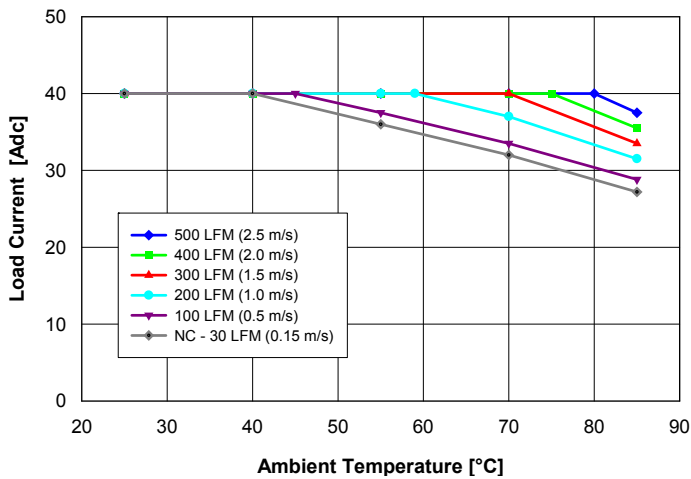
Fig. 1.2V.1: Available load current vs. ambient air temperature and airflow rates for QM48T40012 converter with B height pins mounted vertically with air flowing from pin 3 to pin 1, MOSFET temperature \leq 120^\circ\text{C} , V_{in} = 48\text{ V} .
