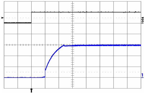
Fig. 1.5V.8: Turn-on transient at full rated load current (resistive) plus 40,000 \mu F at V_{in} = 48 V, triggered via ON/OFF pin. Top trace: ON/OFF signal (5 V/div.). Bottom trace: output voltage (0.5 V/div.). Time scale: 2 ms/div.
