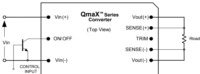
Fig. A: Circuit configuration for ON/OFF function.
