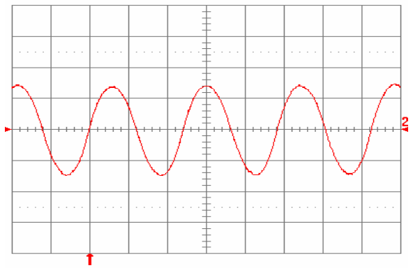
Fig. 2.5V.13: Input reflected ripple current, i_c (100 mA/div), measured at input terminals at full rated load current and V_{in} = 48 V. Refer to Fig. 2.5V.11 for test setup. Time scale: 1 μs/div.
